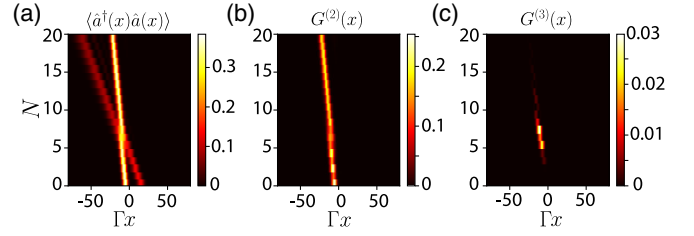
FIG. 4. Evolution of the state |\text{in}\rangle (see text) demonstrating the interaction between a two-photon bound state centered at a_2 = -10/\Gamma and a single photon centered at a_1 = 15/\Gamma both with width \sigma\Gamma = 3\sqrt{2} . The output observables (a) \langle \hat{a}^\dagger(x) \hat{a}(x) \rangle , (b) G^{(2)}(x) , and (c) G^{(3)}(x) are plotted versus the number of emitters N .
