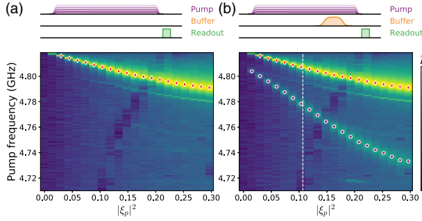
FIG. 6. Complete spectroscopic data. (a),(b) The excited state population of the qubit p_e (color coded) is represented as a function of the pump amplitude ( x axis) and pump frequency ( y axis). (a) When there is no incoming photon on the buffer port, we find one spectroscopic line (red diamonds) for which the qubit is sent into its excited state. This corresponds to a higher-order amplification process of the form. We also observe that the background p_e is rising approximately linearly with the pump power at all the frequencies, which is consistent with the heating of the qubit bath by the pump. (b) When we add a pulse on the buffer port at frequency \omega_b , another line (purple circles) appears. This line corresponds the process \hat{b}\hat{\sigma}^\dagger\hat{w}^\dagger and the white dashed line indicates the chosen pump power which maximizes the ratio \eta/\Gamma_{\text{dc}} . We can also observe a spectroscopic line which goes upward which seems to cool the qubit and thus decreases the efficiency [see dip in \kappa_{\text{nl}} in Fig. 1(a)]. This was the main reason for limiting the pump power to the chosen value. Also, past this line, the dark count rate increases too much compared to the gain in the efficiency.
