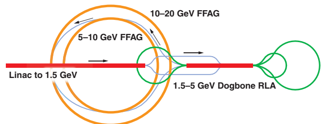
FIG. 19. (Color) Potential layout for the acceleration systems.
