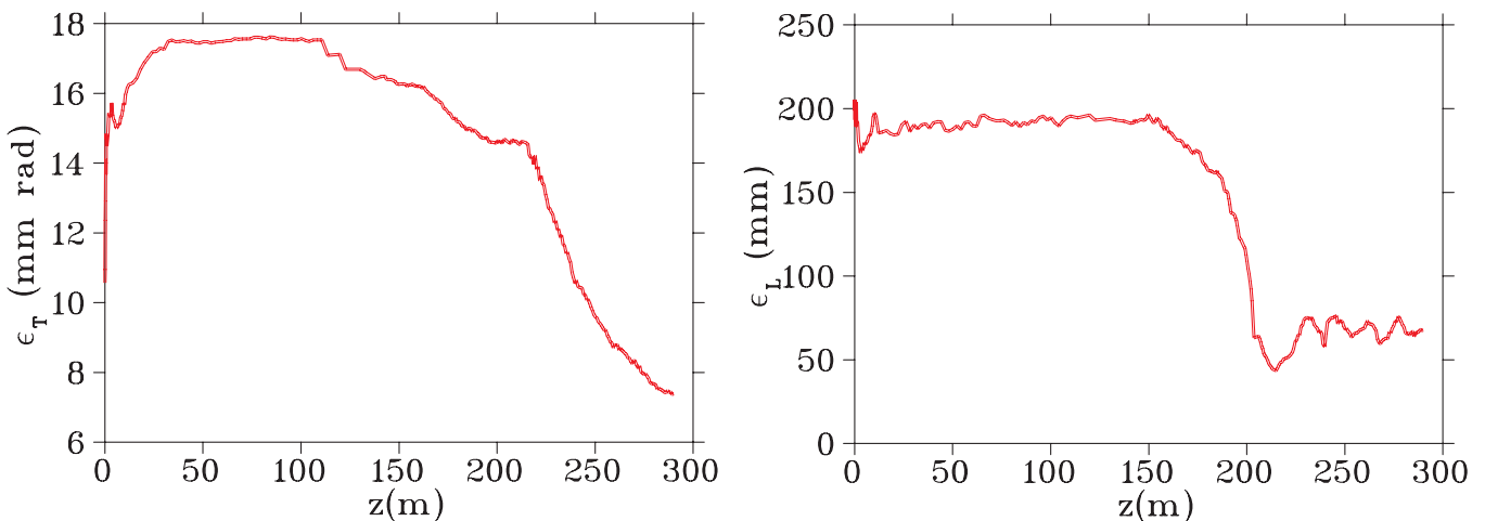
FIG. 14. (Color) Normalized transverse emittance (left) and longitudinal emittance (right) along the front end for a momentum cut 0.1 \leq p \leq 0.3 \text{ GeV}/c .
