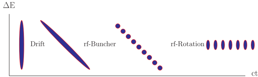
FIG. 2. (Color) Comparison of the buncher concept used here (bottom) with the bunching system used in FS2 (top).
