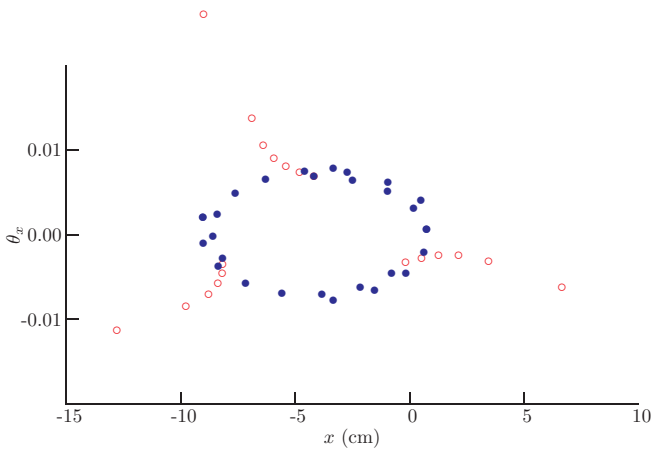
FIG. 33. (Color) Horizontal phase space from tracking at 5.1 GeV/ c at the outer edge of the acceptance. Open circles are without the body sextupole fields and show a third-order resonance; filled circles are with the body sextupole fields.
