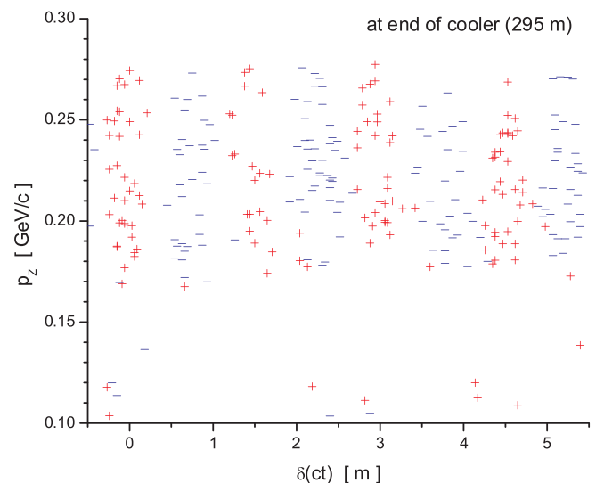
FIG. 18. (Color) A sample from the train of interleaved \mu^+ (red) and \mu^- (blue) bunches exiting the cooling section.
