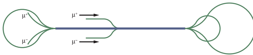
FIG. 23. (Color) Dog-bone (top) and racetrack (bottom) layout for the RLA.
