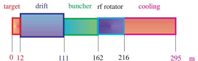
FIG. 4. (Color) Overall layout of the front end.
