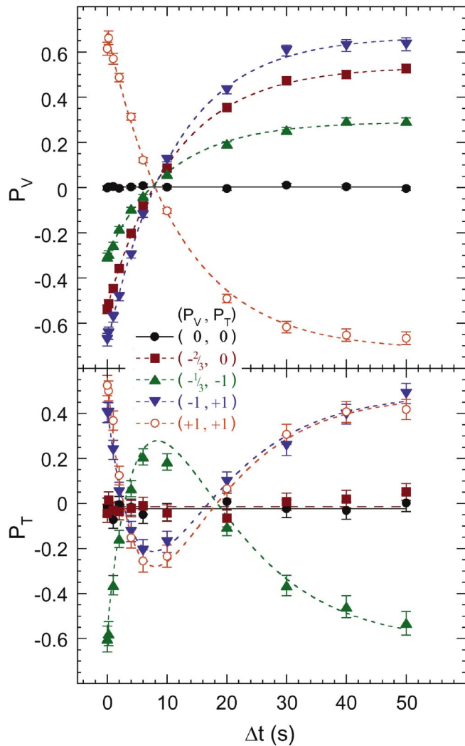
FIG. 4. (Color) The measured vector and tensor deuteron polarizations at 1850 MeV/c are plotted against the rf dipole ramp time \Delta t . The rf dipole's frequency half-range \Delta f/2 was 100 Hz, and its \int B_{\text{rms}} dl was 0.54 T mm. The top and bottom curves are fits using Eqs. (9) and (11), respectively.
