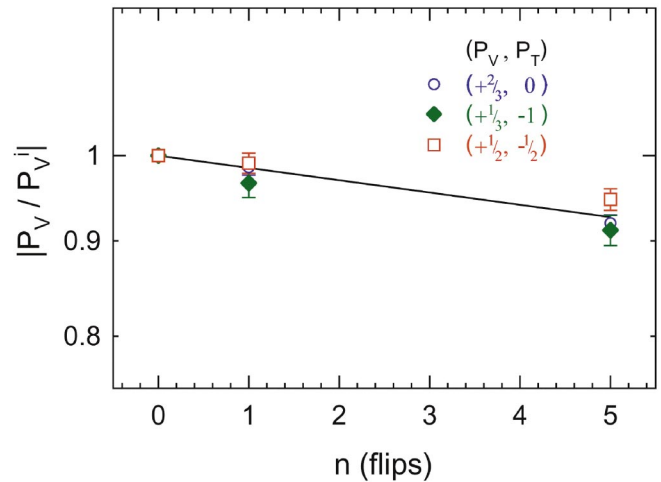
FIG. 9. (Color) The measured vector deuteron polarization ratios at 1850 MeV/ c are plotted against the number of frequency sweeps. The rf dipole's frequency ramp time \Delta t was 60 s; its frequency half-range \Delta f/2 was 75 Hz, and its \int B_{rms} dl was 0.60 T mm. The line is a fit using Eq. (16).
