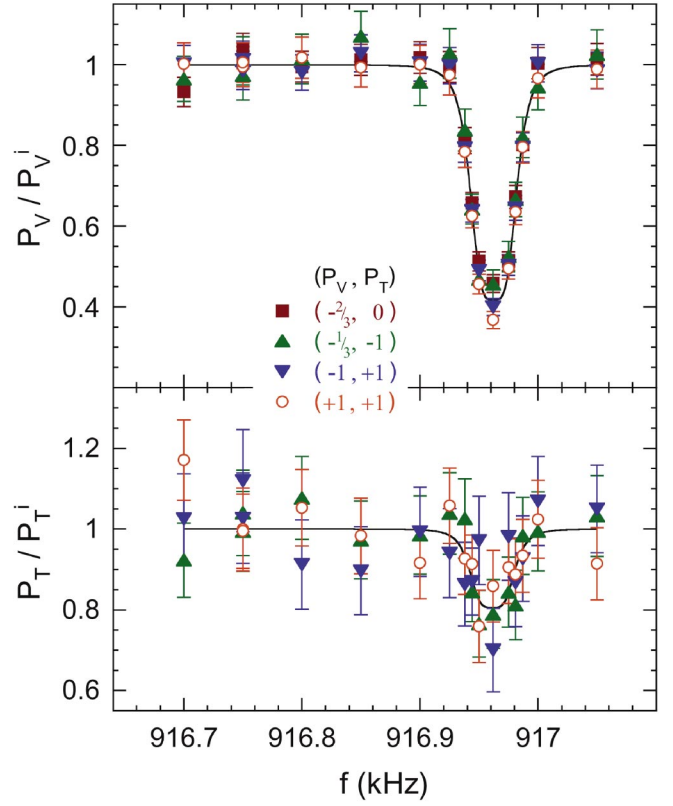
FIG. 3. (Color) The measured vector and tensor deuteron polarization ratios at 1850 MeV/ c are plotted against the rf dipole's fixed frequency. The P_V^i and P_T^i are the average of the six points furthest from the deep for each curve. The rf dipole's \int B_{\text{rms}} dl was 0.54 T mm. The curves are second-order Lorentzian fits.
