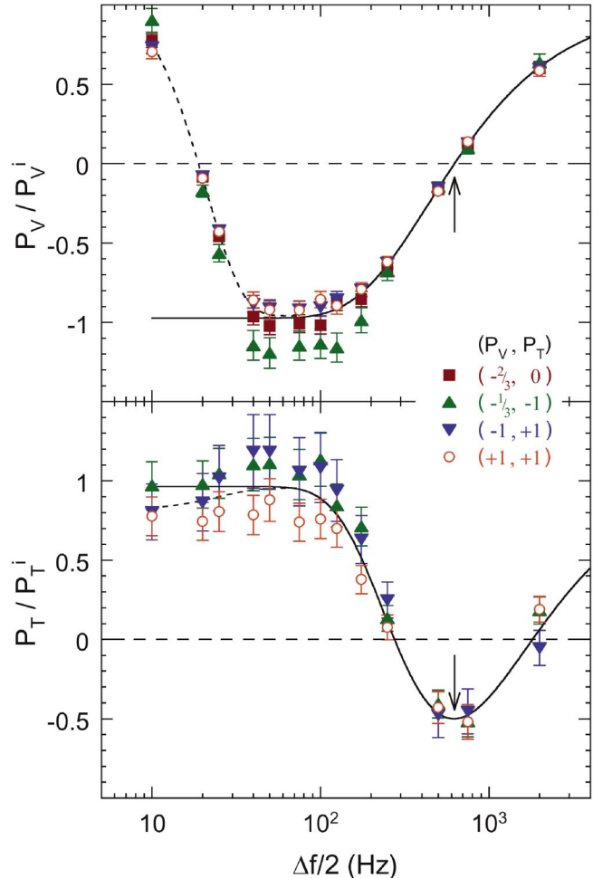
FIG. 7. (Color) The measured vector and tensor deuteron polarization ratios at 1850 MeV/c are plotted against the rf dipole's frequency half-range \Delta f/2 . The P_V and P_T were obtained from fits to the data as shown in Table III. The rf dipole's ramp time \Delta t was 50 s, and its \int B_{\text{rms}} dl was 0.54 T mm. The top and bottom solid curves are fits to the data for all states at and above \Delta f/2 = 75 Hz using Eqs. (9) and (11), respectively. The dashed lines are to guide the eye. The arrows mark a 90^\circ rotation where P_V = 0 and P_T = -\frac{1}{2}P_T^i .
