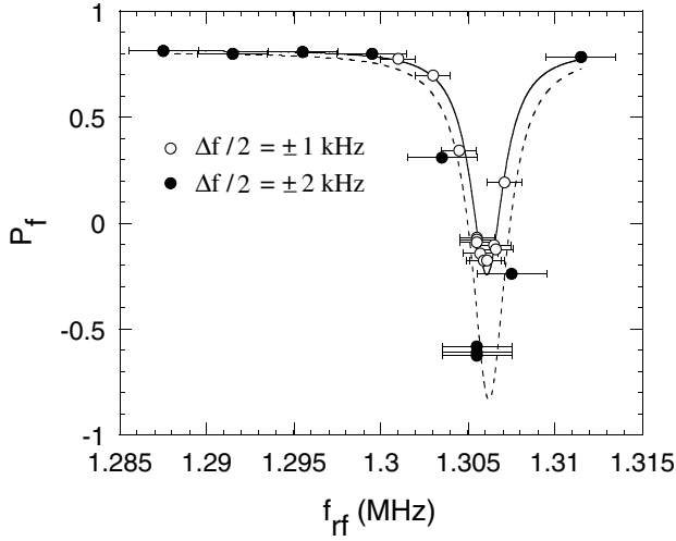
FIG. 2. The measured proton polarization at 1.941 GeV/c is plotted against the central frequency of each ramp; each ramp's \Delta f range is shown by a horizontal bar. The rf dipole's \int B_{\text{rms}} dl was 0.11 T mm; its \Delta t was 10 s. The curve is a fit using a first-order Lorentzian.
