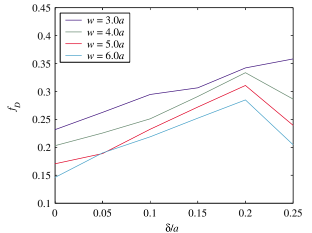
FIG. 7. (Color) Damage factors of various structure geometries.
