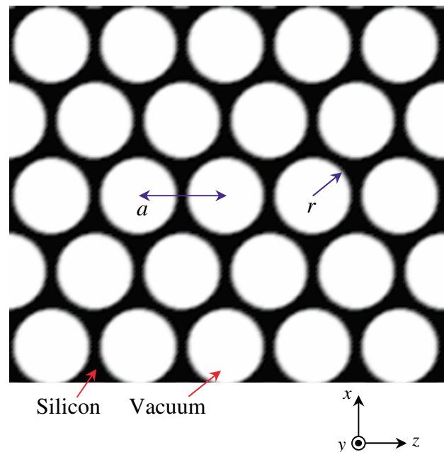
FIG. 1. (Color) The geometry of an optimized 2D photonic crystal lattice consisting of vacuum holes in silicon. Here r = 0.427a . The coordinate system used throughout this paper is shown, and we take the particle beam to propagate in the z direction.
