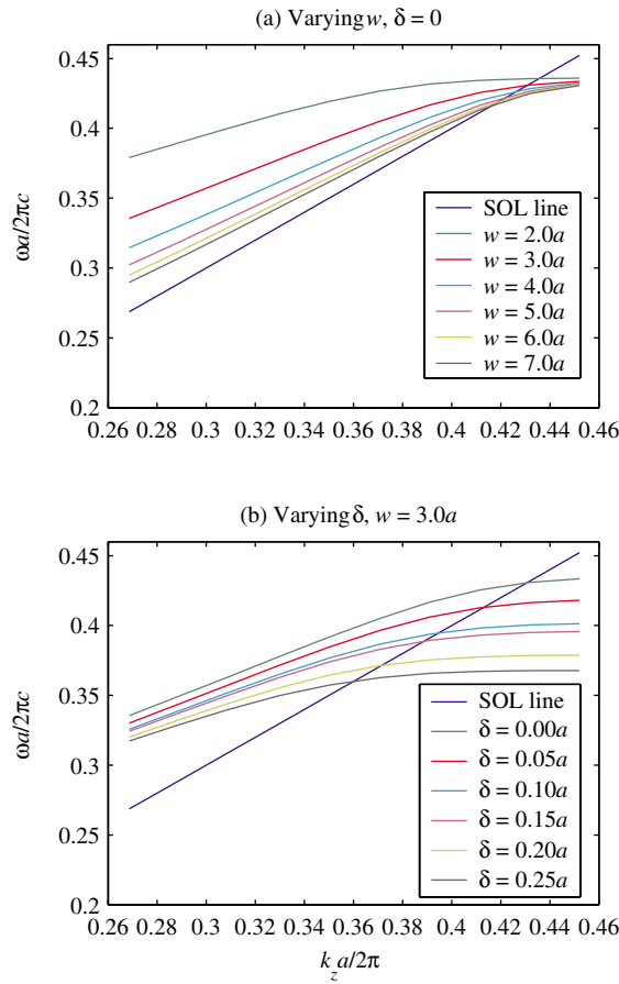
FIG. 4. (Color) Dispersion curves for a set of waveguide geometries, plotted with the speed-of-light (SOL) line shown. The range of wave numbers consists of all k_z with ck_z a frequency in the band gap. (a) We fix \delta = 0 and vary w ; (b) we fix w = 3.0a and vary \delta .
