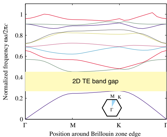
FIG. 2. (Color) The TE band structure of the photonic crystal lattice shown in Fig. 1, with r = 0.427a . The symbols \Gamma , M , and K refer to the points at the corners of the irreducible Brillouin zone, as shown in the inset.
