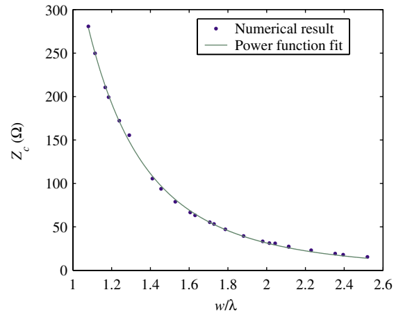
FIG. 6. (Color) Characteristic impedances of 2D photonic crystal waveguide structures. By normalizing the impedance to that of a structure one wavelength high, we obtain a value of Z_c in \Omega . The data shown here include multiple values of \delta ranging from 0 to 0.25a .
