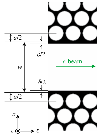
FIG. 3. (Color) The waveguide design, illustrating the geometric parameters. Here r = 0.427a , w = 3.0a , and \delta = 0.25a .
