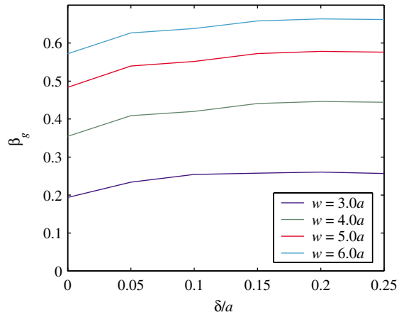
FIG. 8. (Color) Group velocities of accelerating modes for a variety of w and \delta/a values.
