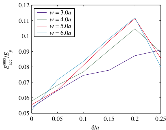
FIG. 9. (Color) The maximum accelerating gradient sustainable by each structure geometry, normalized to the material damage threshold E_p for 1 ps pulses. We assume a structure length of 25 mm.
