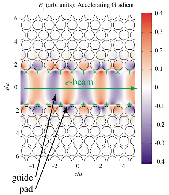
FIG. 5. (Color) An accelerator structure geometry with a speed-of-light waveguide mode. The circles delineate the vacuum holes, and the blue/red coloring denotes the accelerating E_z component. Here w = 3.0a and \delta = 0.25a , and for this mode \lambda = 2.78a . The asterisks show the damage sites, where the field magnitude in the dielectric is maximized.
