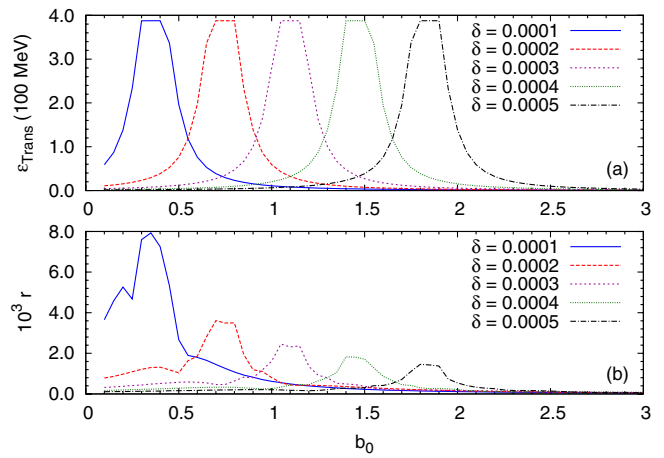
FIG. 9. Maximum energy (a) and radius of the particle orbit in dimensionless units (b) as a function of magnetic field for different values of detuning parameter \delta with phase modulation parameter \alpha = 0.5 .
