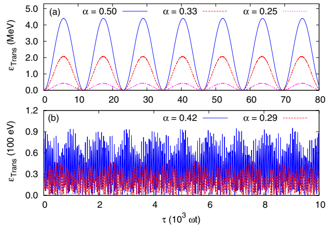
FIG. 3. Temporal evolution of transverse kinetic energy of proton for (a) three different phase modulation factor \alpha = 1/n with n = 2, 3 , and 4 being an integer; similarly the case when n is not an integer is also presented (b). The amplitude of the EM wave a_0 = 0.1 and constant magnetic field along wave propagation b_0 = 1.0 is considered.
