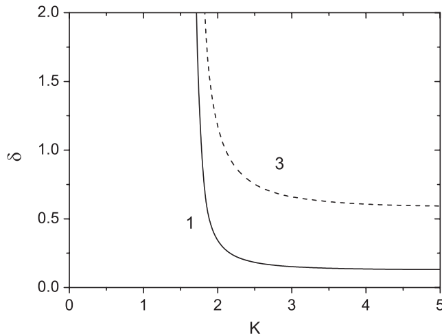
FIG. 3. Parameter \delta for the retuned fundamental harmonic ( \delta^{(1)} , solid line), and for the third harmonic ( \delta^{(3)} , dashed line), versus rms undulator parameter. The gain lengths of the third harmonic and of the retuned fundamental harmonic are equal. Retuning is done by reducing undulator parameter.
