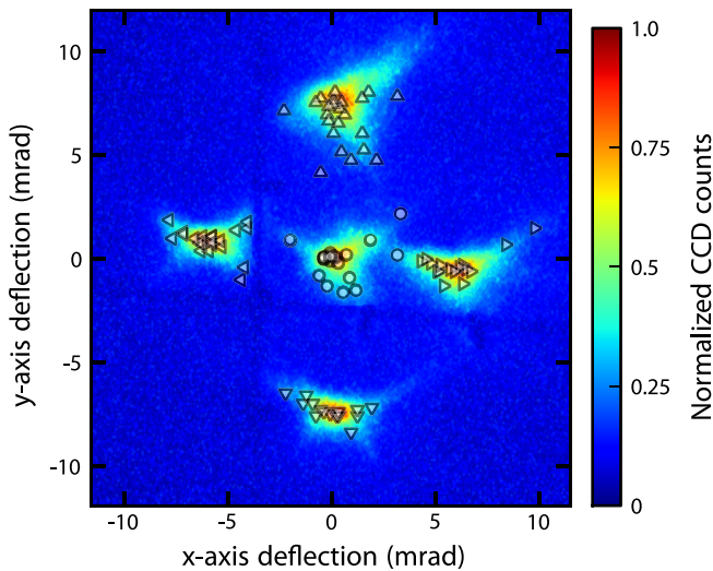
FIG. 5. Electron beam steering: False color summed images observed at S1, 1.12 m behind the electron source with symbols marking the peak position of individual shots. The central spot shows the sum of 18 shots (circles). The surrounding four spots (triangles of differing orientation) were observed after offsetting the second lens transversely to the beam propagation direction in four separate positions. This introduces a dipole moment which deflects the electron beam. The lens was moved by \pm 390 \mu\text{m} and \pm 530 \mu\text{m} in the x and the y directions and caused corresponding angular deflections of 6.1 and 7.3 mrad in the same direction.
