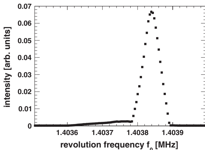
FIG. 2. Mean Schottky power spectrum extracted from measurements over five days at one energy. The statistical error bars lie within the data points. By calculating the weighted arithmetic mean, an average revolution frequency of \bar{f}_0 = 1\,403\,831.75 \pm 0.12 Hz was deduced.
