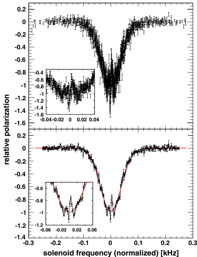
FIG. 4. (Color) Panel (a): The spin-resonance spectra normalized by a Gaussian. Panel (b): The same but with larger bins. The spin-resonance shape is symmetric about zero and smooth except in the center, where a double peak structure is seen. The structures, especially the double peak in the center, are caused by the interaction of the deuteron beam with the bb cavity. The insets show the resonance valley in greater detail.
