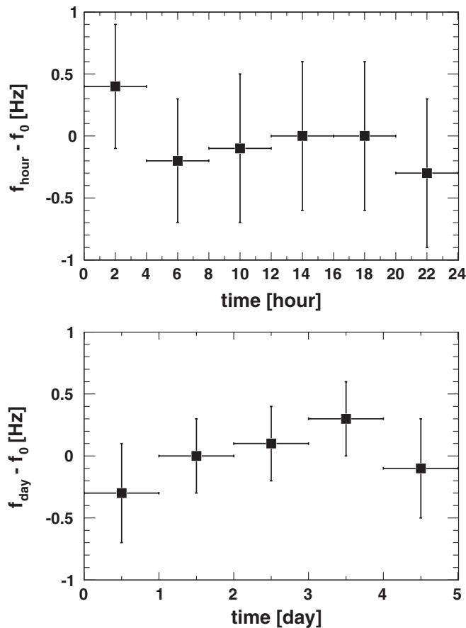
FIG. 5. Stability of the revolution frequency f_0 . In panel (a) the differences between the revolution frequencies for every four hours and the mean revolution frequency of the day are shown. In panel (b) the differences between the revolution frequencies for each day and the mean revolution frequency of the five days of Schottky data taking are shown. From these figures it is clear that the revolution frequency at COSY is very stable, with variations below 1 Hz at a circulation frequency of f_0 \approx 1.4 MHz.
