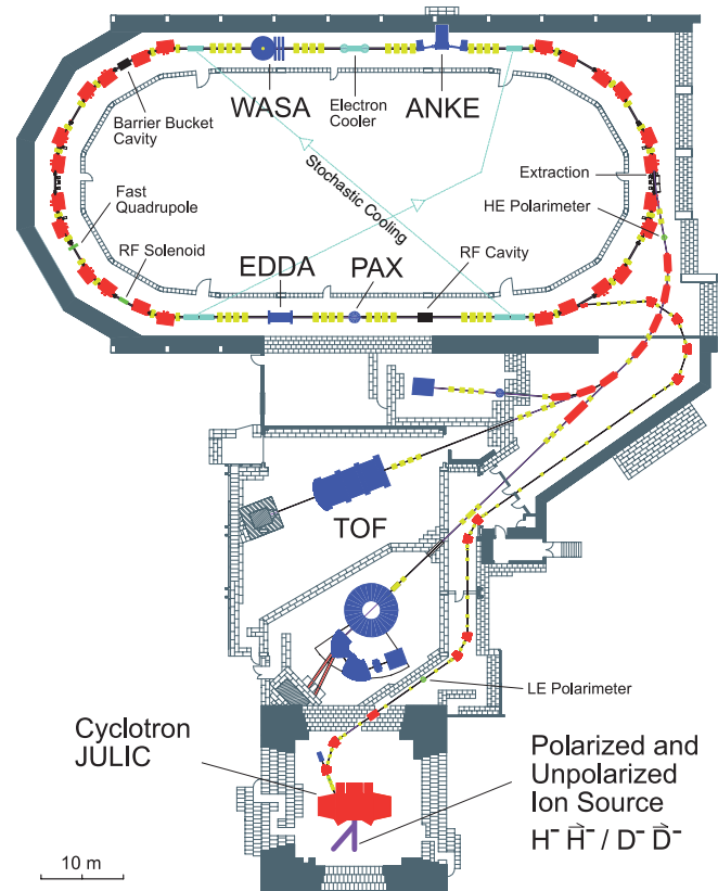
FIG. 1. (Color) The COSY accelerator facility. The cyclotron JULIC provides both unpolarized and polarized proton and deuteron beams for injection into the COSY ring, where they are accelerated and stored. COSY operates in the momentum range of 300–3700 MeV/c. The position of the ANKE spectrometer with the thick internal hydrogen cluster-jet target is shown, as are those of the rf solenoid to depolarize the deuteron beam, the barrier bucket cavity to compensate beam-target energy losses, and the EDDA detector that was used as a beam polarimeter.
