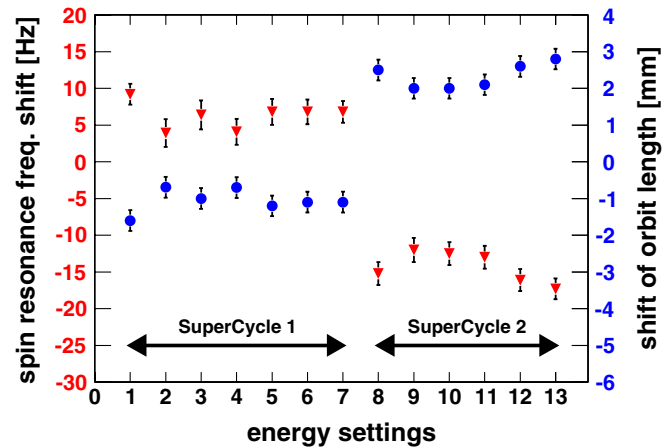
FIG. 6. (Color) The spin-resonance frequencies were measured twice, once before and once after the five days of data taking. The red triangles present the shift of the spin-resonance frequency f_r from the first to the second measurement. These shifts correspond to changes in the orbit length, which are shown as blue circles. For the first supercycle, the spin-resonance frequencies decrease between the two measurements by 4–10 Hz, which corresponds to an increase in the orbit length in the range of 0.7–1.6 mm. For the second supercycle an increase of the spin resonance in the range of 12–17 Hz was observed, i.e., a decrease in the orbit length in the range of 2.0–2.8 mm.
