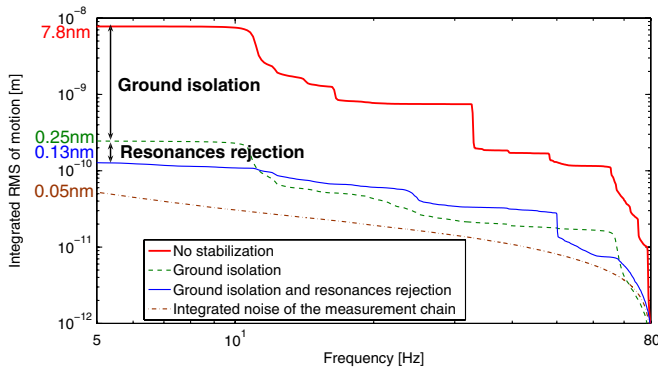
FIG. 9. (Color) Demonstration of stabilization to the subnanometer level via ground isolation and structure resonance rejection in a quiet environment [45].
