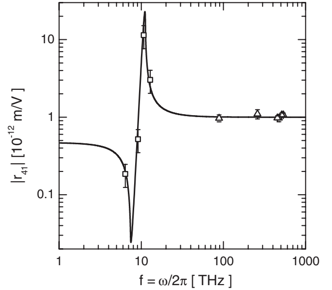
FIG. 8. Absolute magnitude of the EO coefficient r_{41}(\omega) of GaP. The square symbols \square are experimental data taken from Ref. [17], the triangles \triangle from Ref. [33]. The curve is a fit of the experimental data using Eq. (24) with the parameters shown in the text.
