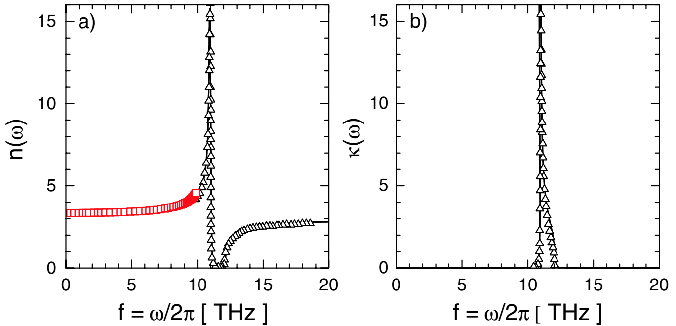
FIG. 6. (Color) (a) Real part n(\omega) and (b) imaginary part \kappa(\omega) of the refractive index of GaP. Here the lowest TO resonance is at 11 THz. The triangles \triangle are experimental data taken from Ref. [30], the squares \square from Ref. [23]. The curves are fits of the experimental data using the formulas and the parameters shown in the text.
