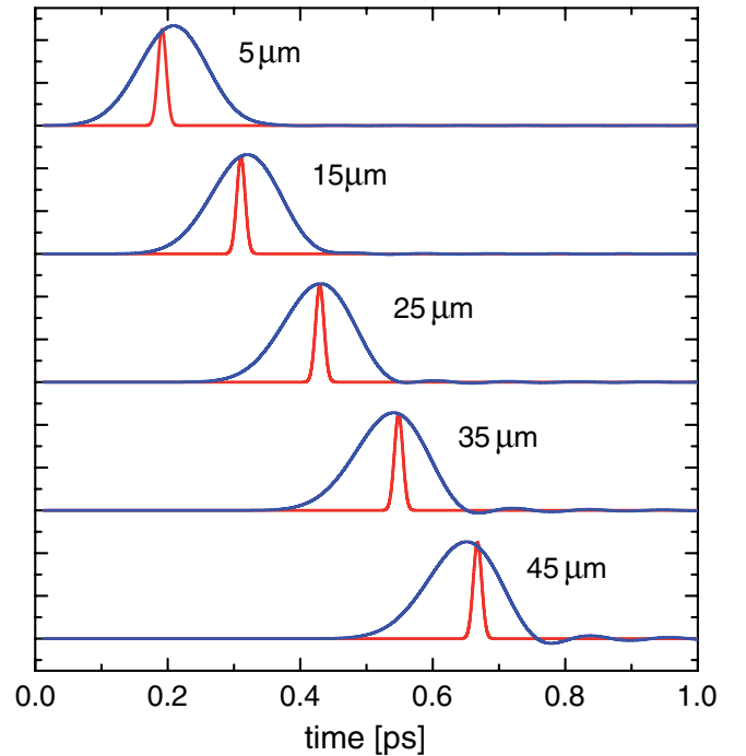
FIG. 12. (Color) Computed propagation of a Gaussian THz pulse with an initial rms width of \sigma = 50 \text{ fs} in a 50 \mu\text{m} thick GaP crystal. The blue curves show the time profiles at selected positions in the crystal ( z_j = 5, 15, 25, 35, 45 \mu\text{m} ). The positions of the laser pulses are shown as well (narrow red curves).
