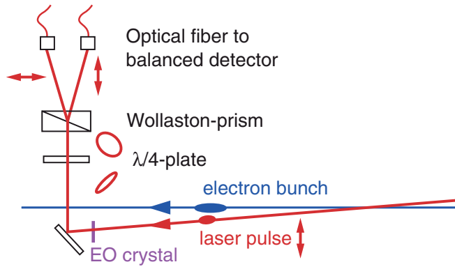
FIG. 4. (Color) Simplified top view of electro-optic signal detection using a quarter wave plate, a Wollaston prism, and a balanced diode detector. The incident laser beam is polarized horizontally. The quarter wave plate is rotated by 45^\circ with respect to the horizontal plane.
