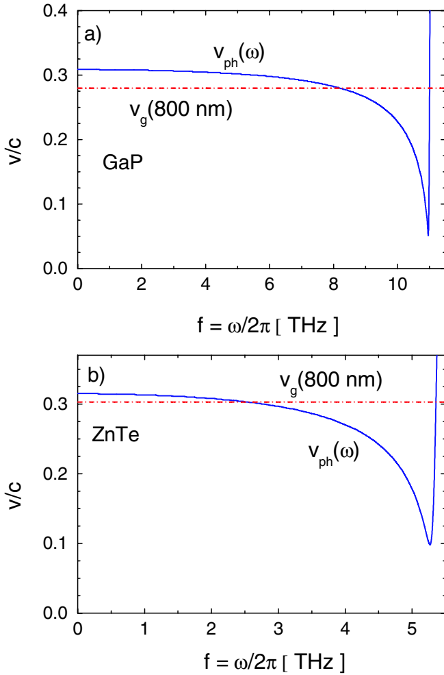
FIG. 11. (Color) (a) Phase velocity of GaP in the THz range. The optical group velocity at \lambda = 800 \text{ nm} is shown as a dash-dotted line. The velocities have been divided by c . (b) THz phase velocity and optical group velocity of ZnTe.
