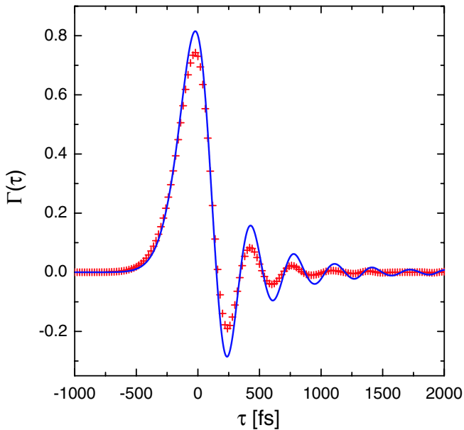
FIG. 17. (Color) Effect of laser-pulse broadening in a 500 \mu\text{m} thick ZnTe crystal which is placed at a distance r = 5 mm from an electron beam with bunch charge Q = 0.1 nC and rms bunch duration \sigma_i = 70 fs. Plotted is the phase retardation \Gamma(\tau) as a function of the relative delay \tau between the THz pulse and the laser pulse. Continuous blue curve: delta-function-like laser pulse, Eq. (38). Crosses: laser-pulse broadening taken into consideration according to Eq. (40). The initial laser-pulse length is \sigma_0 = 6.4 fs.
