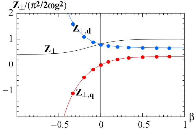
FIG. 15. (Color) For an elliptical step-out transition to a large beam pipe, the leading order dependence of the transverse impedances Z_{\perp} , Z_{\perp,d} , Z_{\perp,q} , normalized to \pi^2/(2\omega g^2) , as functions of \beta = (w - g)/(w + g) . The plotting symbols give ECHO numerical results for comparison.
