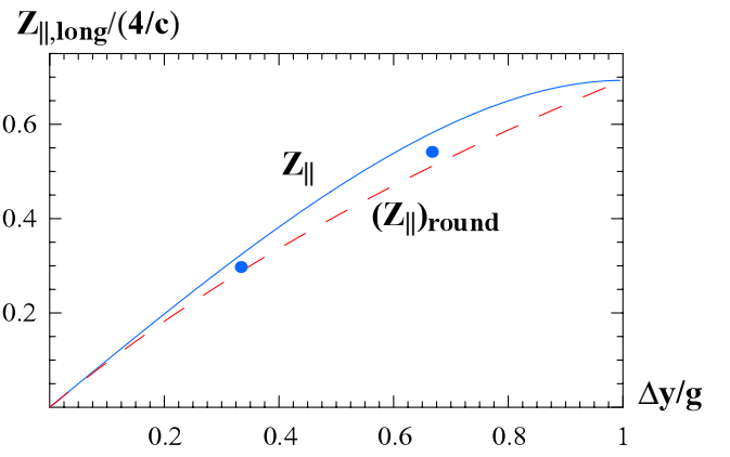
FIG. 19. (Color) For the misaligned, flat pipe of aperture 2g , the longitudinal impedance Z_{\parallel,long} as a function of misalignment parameter \Delta y/g . Plotting symbols give ECHO results. As a scale comparison, the impedance of a round, step-out transition, from radius g to radius g + \Delta y , (Z_{\parallel})_{\text{round}} = 4 \ln(1 + \Delta y/g)/c , is also given (dashes).
