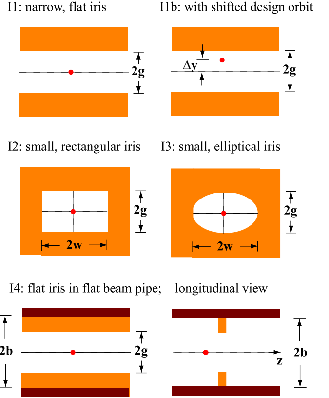
FIG. 6. (Color) Cross-section views of the iris/short collimator geometries considered in this section (for case I4 a longitudinal view is also given). Dimension labels are given, and the design orbit location is indicated by the red dot. In cases I1–I3, the beam pipe aperture is specified as large compared to the iris aperture; in case I4 the beam pipe is flat, with vertical aperture 2b . For case I4 two colors are used for the boundaries as an aid in visualization.
