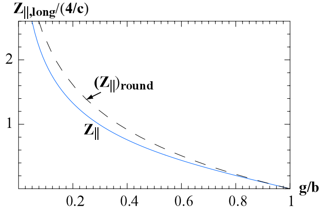
FIG. 10. (Color) For a thin flat iris with aperture 2g in a flat beam pipe of aperture 2b , the longitudinal impedance Z_{||,long} as function of \alpha = g/b . The round case, (Z_{||})_{round} = 4 \ln(b/g)/c , is also shown (dashes).
