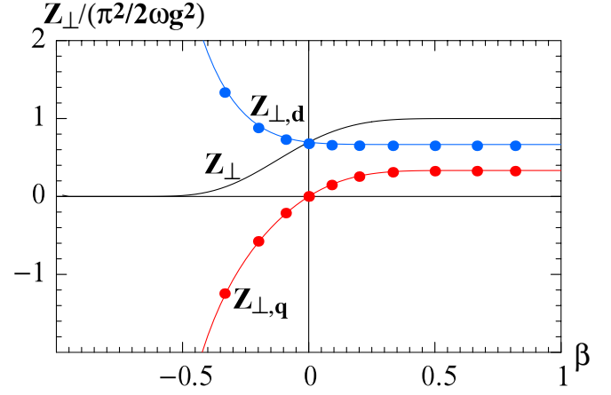
FIG. 14. (Color) For a rectangular step-out transition to a large beam pipe, the leading order dependence of the transverse impedances Z_{\perp} , Z_{\perp,d} , Z_{\perp,q} , normalized to \pi^2/(2\omega g^2) , as functions of \beta = (w-g)/(w+g) . The plotting symbols give ECHO numerical results for comparison.
