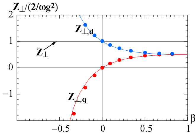
FIG. 8. (Color) For an elliptical iris in a beam pipe, the transverse impedances Z_{\perp} , Z_{\perp,d} , Z_{\perp,q} , normalized to 2/(\omega g^2) , as functions of \beta = (w - g)/(w + g) . Plotting symbols give ECHO numerical results.
