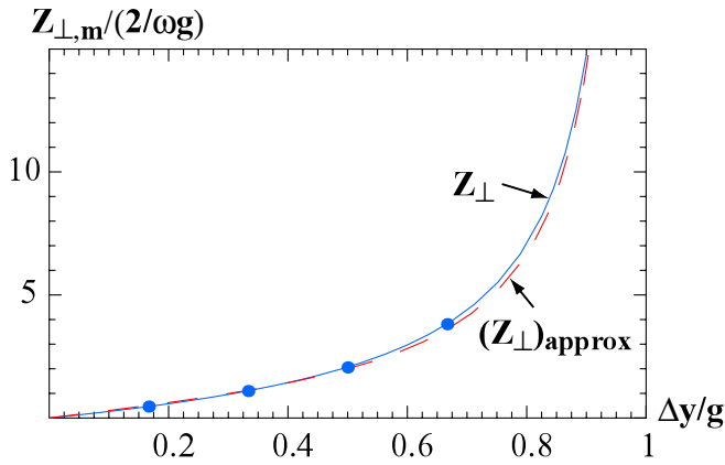
FIG. 18. (Color) For the misaligned, flat pipe of aperture 2g , the transverse impedance Z_{\perp,m} as a function of misalignment parameter \Delta y/g . Plotting symbols give ECHO results. The approximation, (Z_{\perp,m})_{\text{approx}} , is also shown (dashes).
