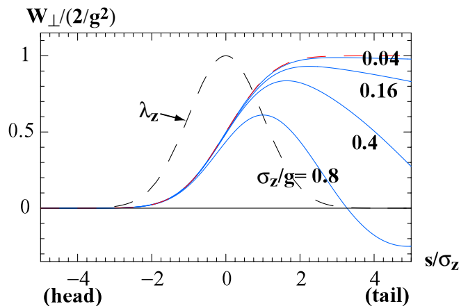
FIG. 4. (Color) Transverse wake of a thin round iris in a beam pipe as obtained by ECHO. Results for bunch lengths over iris radius \sigma_z/g = 0.04, 0.16, 0.4 , and 0.8 are given. The (Gaussian) bunch shape, with the head to the left, is indicated by the black dashes. The analytical wake of a Gaussian bunch in a round iris in the optical regime, W_{\perp} = [1 + \text{erf}(s/\sqrt{2}\sigma_z)]/g^2 , with \text{erf}(x) the error function, is also given (the red dashes).
