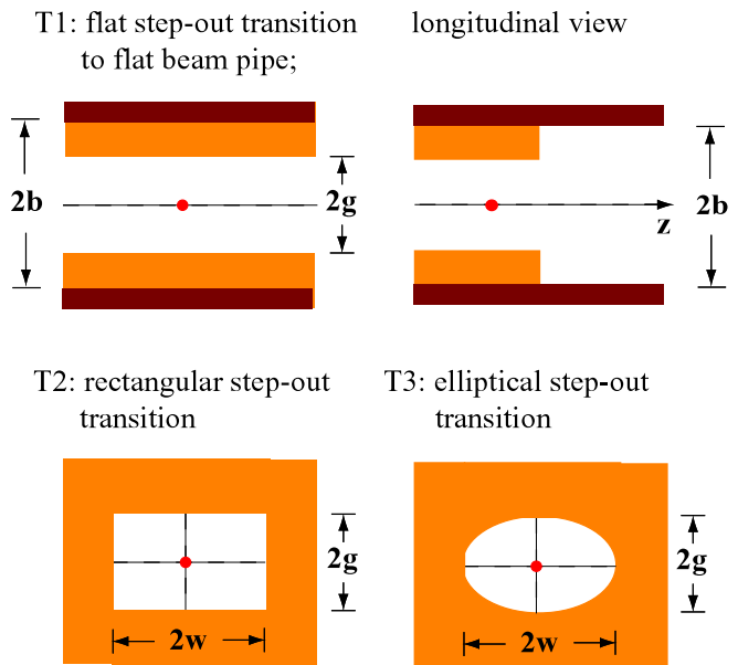
FIG. 12. (Color) Cross-section views of the step-out transition geometries considered in this section (for case T1 a longitudinal view is also given). Dimension labels are given, and the design orbit location is indicated by the red dot. In cases T2–T3 the outgoing beam pipe aperture is specified as large compared to the incoming beam pipe aperture; in case T1 the outgoing beam pipe is flat, with vertical aperture 2b . For case T1 two colors are used for the boundaries as an aid in visualization.
