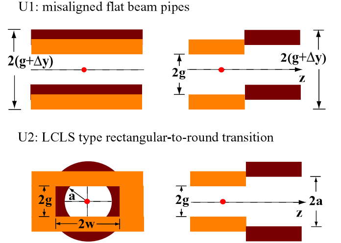
FIG. 16. (Color) Cross-section view (from upstream end; left figures) and longitudinal view (right figures) of more complicated transitions: U1, misaligned flat pipes; and U2, LCLS-type rectangular-to-round transitions. Dimension labels are given; the design orbit location is indicated by the red dot. Two colors are used as an aid in visualization.
