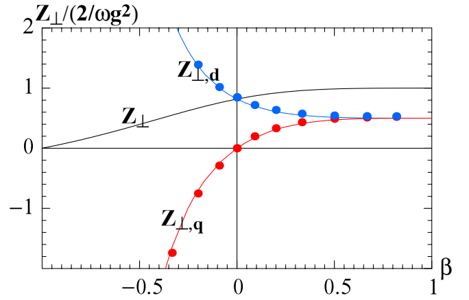
FIG. 7. (Color) For a rectangular iris in a beam pipe, the transverse impedances Z_{\perp} , Z_{\perp,d} , Z_{\perp,q} , normalized to 2/(\omega g^2) , as functions of \beta = (w - g)/(w + g) . Plotting symbols give ECHO numerical results.
