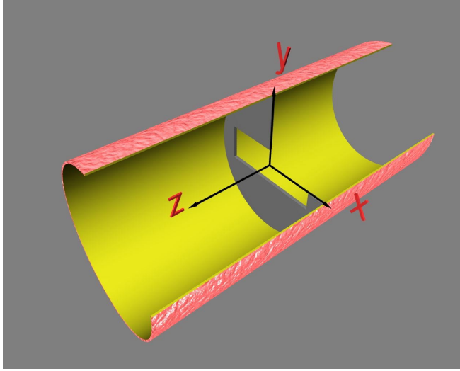
FIG. 5. (Color) An iris in a beam pipe.
