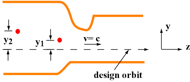
FIG. 2. (Color) Sketch of a transition showing the relationship of the design trajectory and the vertical offsets of particle 1, y_1 , and particle 2, y_2 (the particles are indicated by red dots). For the calculations the offsets y_1, y_2 , are assumed to be small.
