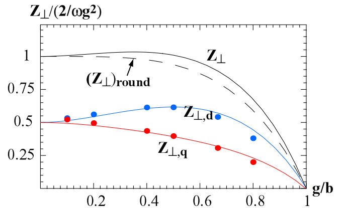
FIG. 9. (Color) For a flat iris with aperture 2g in a flat beam pipe of aperture 2b , the transverse impedances Z_{\perp} , Z_{\perp,d} , Z_{\perp,q} as functions of \alpha = g/b . Plotting symbols give ECHO numerical results. The round case, (Z_{\perp})_{\text{round}} = 2(1/g^2 - g^2/b^4)/\omega , is also shown (dashes).
