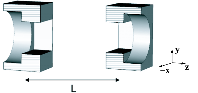
FIG. 17. (Color) A matching pair of LCLS rectangular-to-round transitions in cut-away perspective view. The distance L between transitions is much larger than the catch-up distance for the nominal bunch length.
