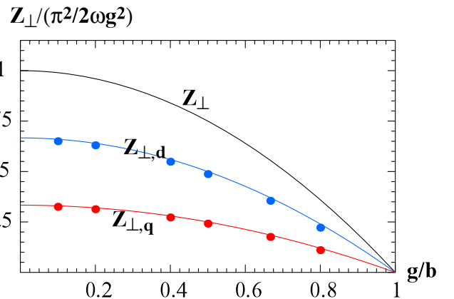
FIG. 13. (Color) For a step-out transition from a flat pipe of aperture 2g into a flat pipe of aperture 2b , the transverse impedances Z_{\perp} , Z_{\perp,d} , Z_{\perp,q} as functions of \alpha = g/b . Plotting symbols give ECHO numerical results for comparison.
