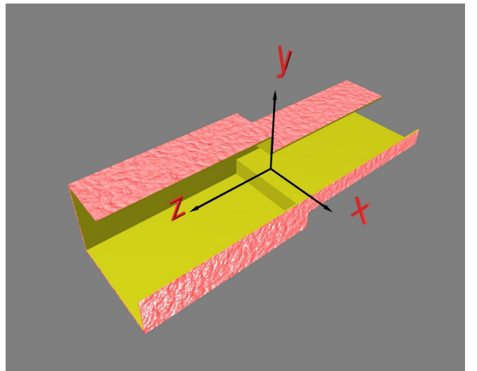
FIG. 11. (Color) A step-out transition. The particles move in the +z direction.
