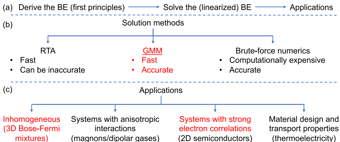
FIG. 1. Overview of the linearized Boltzmann equation and its applications. We develop a solution framework based on Gaussian mixture models (GMM) which enables efficient and accurate analysis of the Boltzmann equation. Applications in red are showcased in this work. We demonstrate the method in detail in the context of trapped Bose-Fermi mixtures of cold atoms—see Fig. 2. Comparisons with experiment are provided in Ref. [5]. We also compute transport coefficients for strongly coupled fermion systems—see Fig. 11. In Ref. [6], we have applied the method to magnon hydrodynamics experiments, computing transport coefficients for systems with anisotropic interactions.
