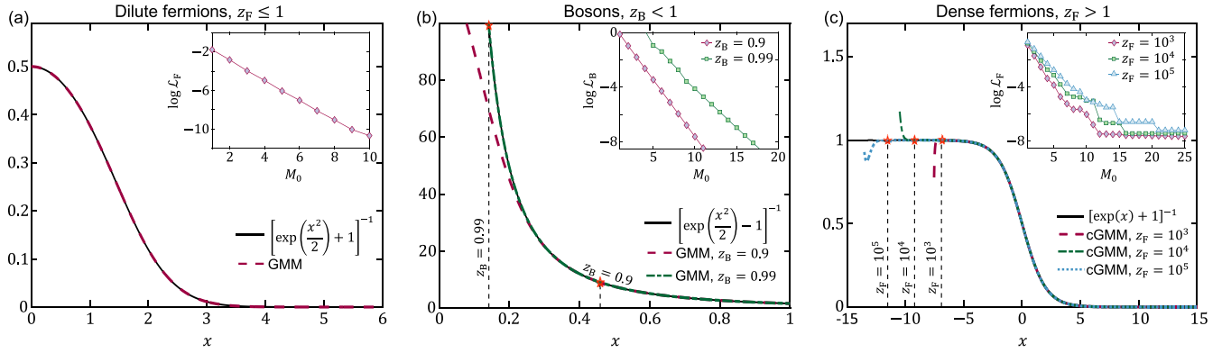
FIG. 3. Performance of the Gaussian mixture model (GMM). (a) The fermionic function f_1(x) (solid line), Eq. (3), that encodes the Fermi-Dirac distribution function for any z_F \leq 1 , and its GMM fit (dashed line) are not distinguishable by eye from each other. The inset shows the dependence of the absolute error of the fit \mathcal{L}_F , Eq. (6), on the total number of Gaussians M_0 that are involved in the fitting: for M_0 = 10 , we obtain \mathcal{L}_F \lesssim 10^{-10} . (b) Similar analysis as in (a) but now we consider the bosonic function f_2(x) (solid line), Eq. (9), in a range x \in [x_{\min}, \infty) , where x_{\min} (vertical dashed lines) is set by the maximal fugacity we consider: x_{\min} \approx 0.46 for z_B = 0.9 and x_{\min} \approx 0.14 for z_B = 0.99 . The GMM fits provide excellent approximations to f_2(x) in their respective domains of applicability (dashed line for z_B = 0.9 and solid dashed line for z_B = 0.99 ): The inset shows that the bosonic error \mathcal{L}_B , Eq. (10), can be as small as 10^{-8} with only about 10 (17) Gaussians for z_B = 0.9 ( z_B = 0.99 ). (c) The fermionic function f_3(x) (solid line), Eq. (13), that captures the Fermi-Dirac distribution function for any 1 \leq z_F \leq z_{\max} , can be well fitted with the complex version of the GMM, Eq. (14). Here, the domain x \in [x_{\min}, \infty) is determined by the maximal fermionic fugacity we consider: x_{\min} = -\ln(z_{\max}) . As shown in the inset, the absolute error of the fit \mathcal{L}_F decreases with increasing the total number M_0 of complex conjugate Gaussian pairs; for M_0 \lesssim 25 , we obtain \mathcal{L}_F \simeq 10^{-8} at z_{\max} = 10^5 .
