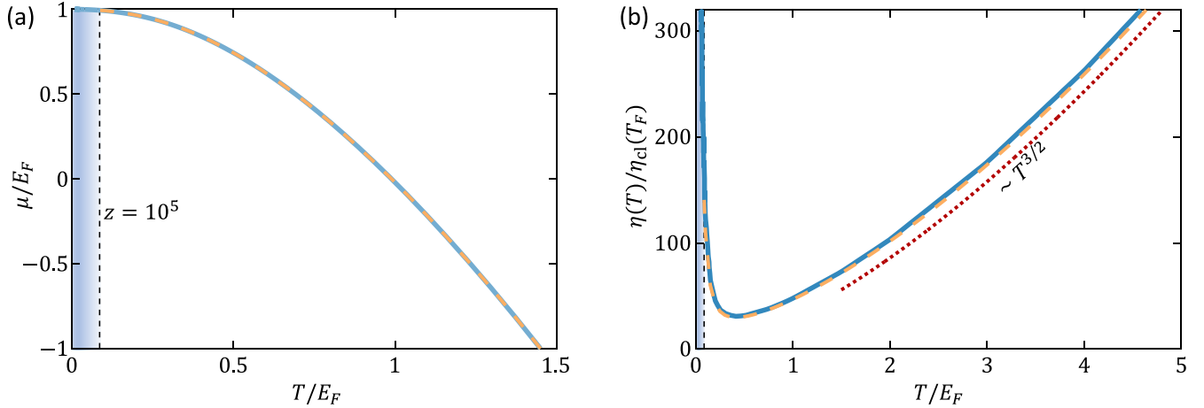
FIG. 11. Performance of the cGMM expansion on a strongly interacting Fermi fluid. (a) The chemical potential \mu as a function of T : The solid line encodes the exact dependence, while the dashed one corresponds to the cGMM. In our simulations, we chose z_{\max} = 10^5 , which implies that the domain of applicability of the cGMM is T \gtrsim 0.1T_F (vertical dashed line), where the two calculation coincide. (b) The shear viscosity \eta of the fluid as a function of T at k_F|a| = 4.5 ( \eta is normalized by \eta_{cl}(T_F) = 5\sqrt{mT_F}/(32a^2\sqrt{\pi}) ). The solid curve is taken from Ref. [89], while the dashed one is obtained using the cGMM, and the two results reasonably agree. The choice k_F|a| = 4.5 implies that T_a \approx 0.1T_F and allows one to see the \sim T^{3/2} scaling (dotted line) at high temperatures, T_F, T_a \ll T . The shaded regions in panels (a) and (b) are where the chosen cGMM is no longer applicable.
