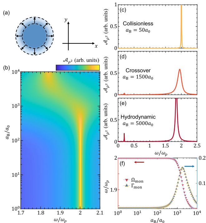
FIG. 4. Collisionless-to-hydrodynamics crossover in a single-component bosonic fluid, the case of monopole mode schematically shown in panel (a). (b) The bosonic spectral response \mathcal{A}_{\rho^2} as a function of frequency \omega and for different interaction strengths, as encoded in a_B . When the Bose-Bose interactions are weak, one gets a sharp response at \omega \simeq 2\omega_\rho ; as a_B is increased, the system starts to exhibit a many-body hydrodynamic response, as evidenced by the fact that first, the spectral function completely broadens but then reforms again into a sharp peak at a frequency notably different from 2\omega_\rho [see also a few cuts shown in panels (c, d, e)]. This is further illustrated in panel (f) as the behavior of the position \Omega_{\text{mon}} and width \Gamma_{\text{mon}} of the peak in panel (b), obtained from a single Lorentzian fit. In the hydrodynamic regime, transverse and longitudinal monopole modes mix, resulting in the emergence of an additional weak peak at the longitudinal frequency \omega \simeq 2\omega_z (e). Parameters used: \omega_z = 2\pi \times 12.2 Hz, \omega_\rho = 2\pi \times 97 Hz, T = 500 nK, N_B = 10^6 , and M = 2 .
