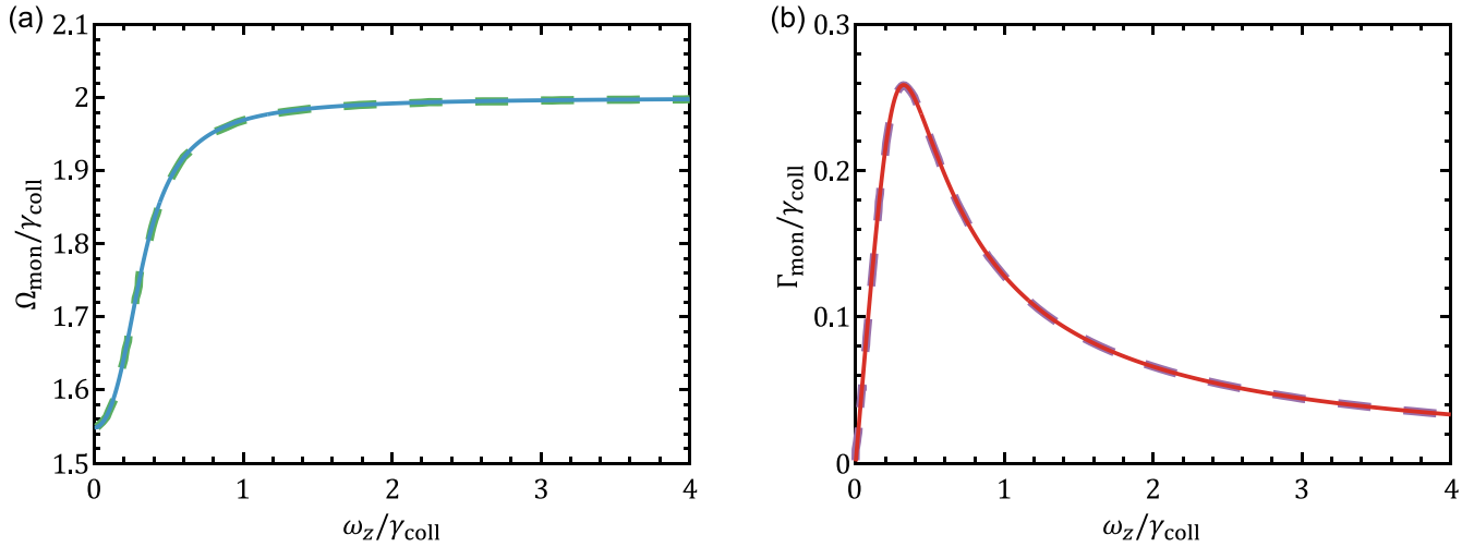
FIG. 9. Monopole mode of a classical gas, trapped into a harmonic potential with \kappa = 10^{-2} . Solid lines in panels (a) and (b) are the monopole mode frequency \Omega_{\text{mon}} and its dampening \Gamma_{\text{mon}} , respectively, computed using the approach developed here. Dashed lines were extracted from Ref. [78]. Similarly to our results in the main text, cf. Fig. 4, the classical gas also exhibits a collisionless-to-hydrodynamic crossover, as evidenced, for instance, by the nonmonotonic behavior of \Gamma_{\text{mon}} .
