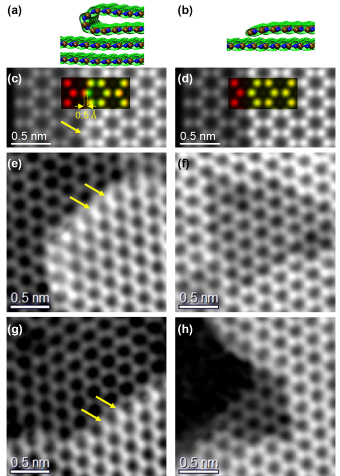
FIG. 2. Simulated and experimental projected potentials of h -BN layers at atomic resolution. (a),(b) Ab initio relaxed structure (blue: N; brown: B) and electron density (green isosurface) from DFT calculations for folded bilayer (a) and monolayer (b) steps. (c),(d) Projections of the DFT potentials along the out-of-plane direction for bilayer step (c) and monolayer step (d). The color-coded insets depicting the separately projected bottom (top) layers in red (green) illustrate the lateral shift of the edge atoms at the bilayer step by 0.5 Å (red-green contrast), which is not present at the single layer step (yellow). (e)–(h) Experimental projected potentials of the white squares in Fig. 1 at which (e) and (g) pertain to the folded bilayer step and (f) and (h) to the monolayer step.
