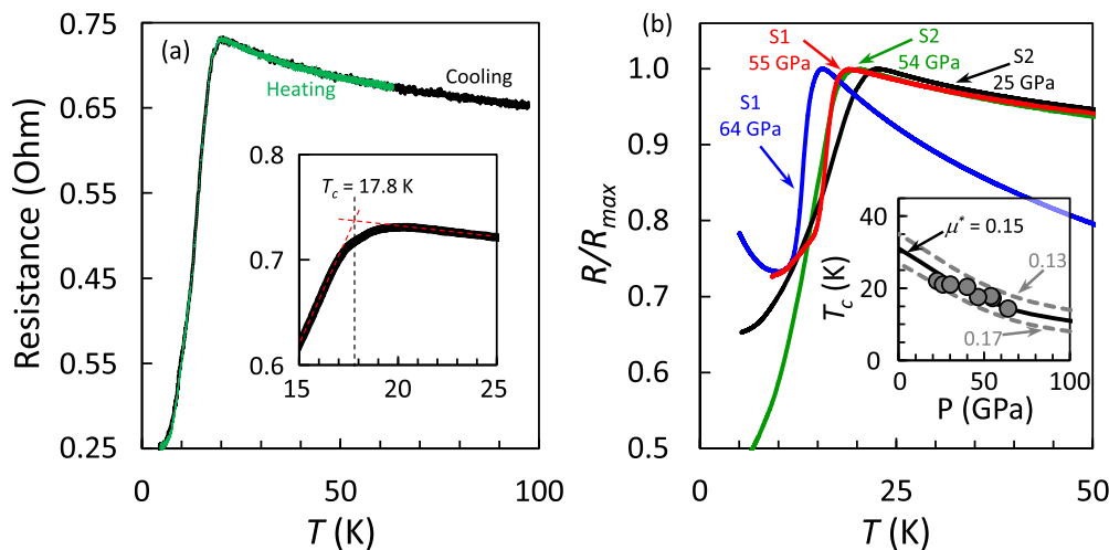
FIG. 3. (a) Resistance drop during cooling of S2 to a base temperature of 5 K at 54 GPa. The heating trace (green overlay) follows the same path with no detectable hysteresis. The inset shows the determination of the T c onset by extrapolation of linear regions. (b) Normalized resistance for several cooling runs at different pressures for samples S1 and S2. The inset shows the pressure dependence of experimental T c onset values for SrB 3 C 3 with pressure (points) compared with calculations using different values of μ* (lines).
