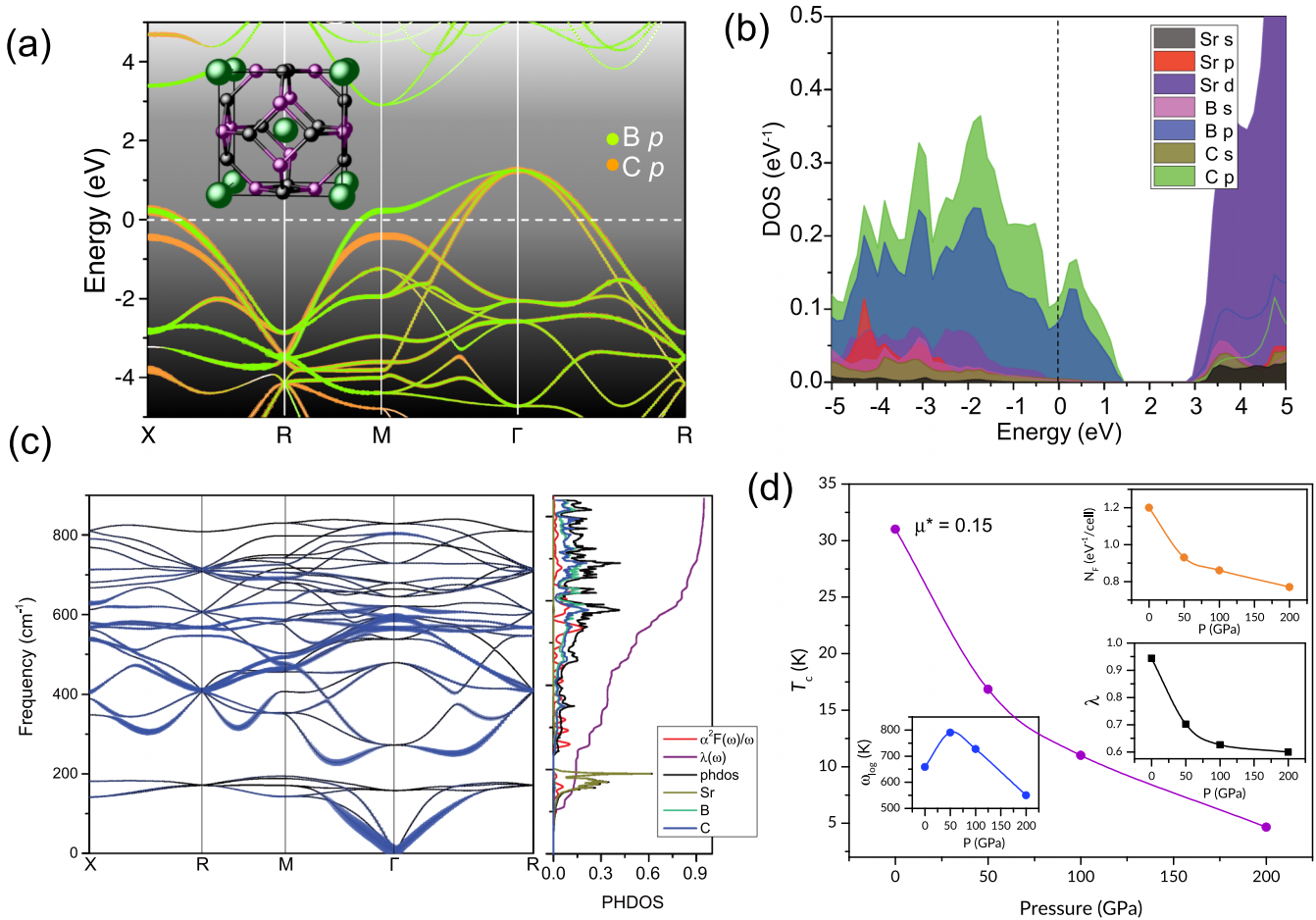
FIG. 1. (a) Electronic band structure for \text{SrB}_3\text{C}_3 at 0 GPa. The bands projected onto the B p and C p orbitals are displayed with green and orange points, respectively. The size of each point is proportional to the weight of the orbital character. The inset shows the crystal structure of the \text{SrB}_3\text{C}_3 clathrate with green, purple, and black spheres representing Sr, B, and C atoms, respectively. (b) Projected DOS in \text{SrB}_3\text{C}_3 . The dashed line indicates the Fermi energy. (c) Phonon dispersion, phonon density of states (PHDOS), phonon spectroscopic function \alpha^2F(\omega)/\omega and electron-phonon integral \lambda(\omega) of \text{SrB}_3\text{C}_3 at 0 GPa. The size of blue circles in the phonon dispersion curves is proportional to the electron-phonon coupling strength. (d) Calculated T_c as a function of pressure with \mu^* = 0.15 . The pressure dependencies of \omega_{\log} , N_F , and \lambda are shown as insets.
