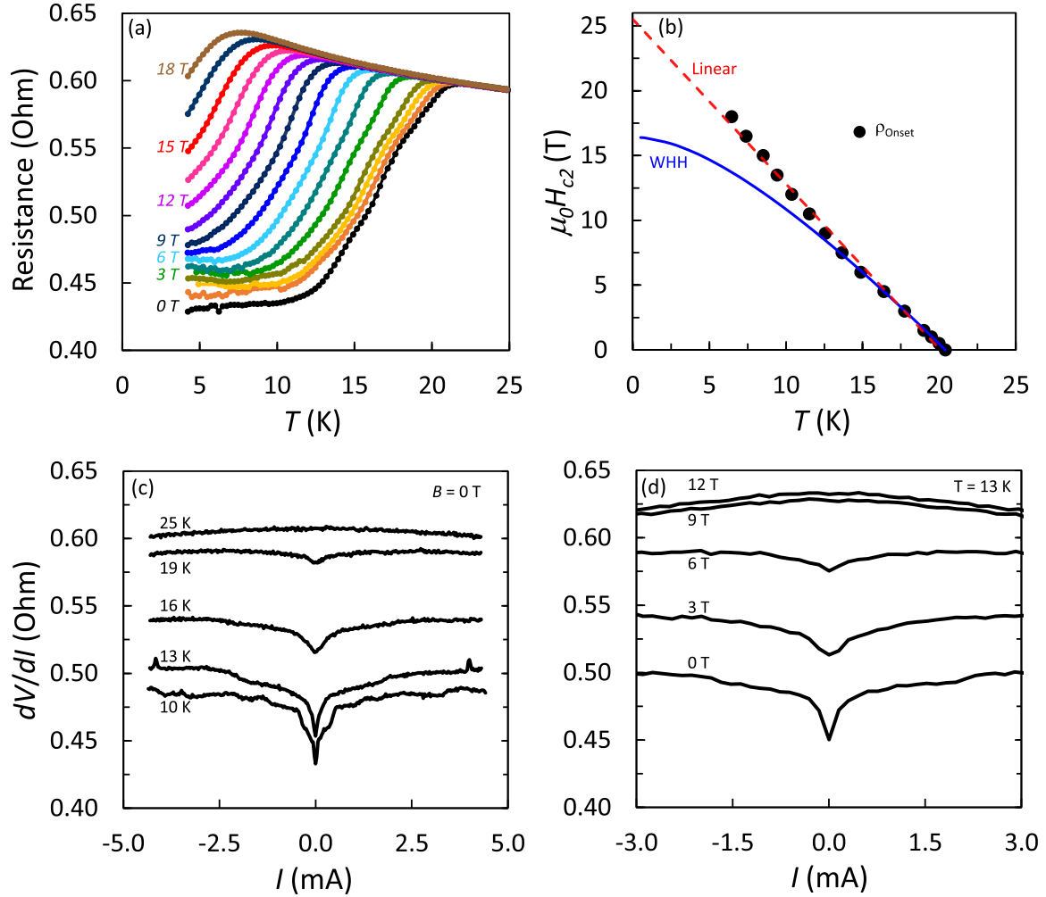
FIG. 4. (a) Resistance of sample S3 at 40 GPa as a function of temperature and magnetic field. (b) \mu_0 H_{c2}(T) for the transition onset (black points) compared with the WHH model ( \alpha = 0 ). A linear fit is shown to guide the eye. Differential resistance measurements performed (c) as a function of temperature at zero field and (d) as a function of field at 13 K. A peak in dV/dI appears at zero bias when T < T_c and B < \mu_0 H_{c2} .
