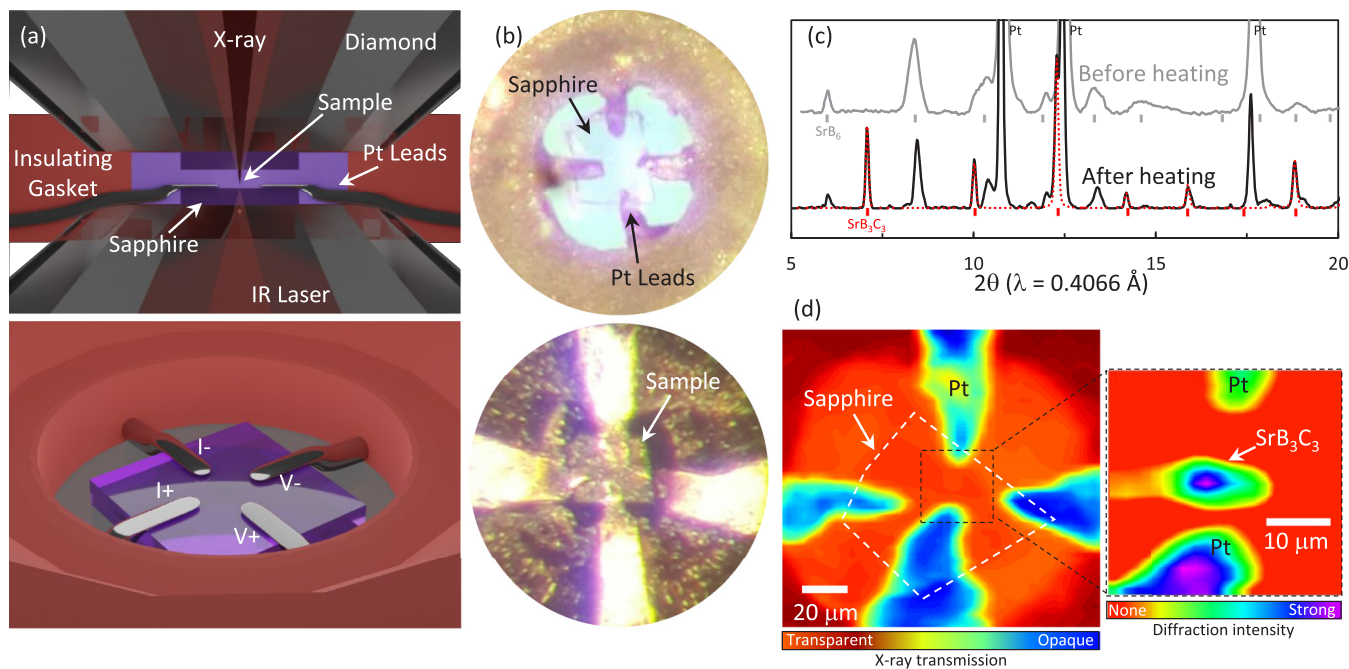
FIG. 2. (a) Sample geometry for in situ electrical transport with HPHT synthesis. The 1Sr:3B:3C precursor is pressed between the diamond anvils, separated by sapphire single crystals that serve as thermal insulation. Four Pt electrical probes sit on the bottom sapphire crystal and are secured within the insulating gasket. (b) Photomicrographs of the sample chamber before loading (view through top diamond), and after loading sample (view through bottom diamond). (c) Representative XRD patterns before and after heating. The heated region shows ~ 60 wt. % SrB 3 C 3 with unconverted cubic SrB 6 . (d) X-ray radiograph of the sample chamber with four Pt wires. Outline of the sapphire is indicated by the white dashed line. The dashed black square contains the laser-heated region between the Pt contacts. The zoom window shows an x-ray-diffraction intensity map for SrB 3 C 3 and Pt showing the synthesized sample between the contacts.
