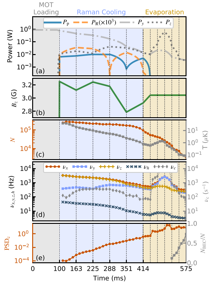
FIG. 2. Control wave forms [panels (a) and (b)] and measured trap and atomic-gas properties [panels (c)–(e)] of the optimized sequence. Gray, blue, and orange shadings mark the MOT loading, Raman cooling, and evaporation periods, respectively. The Raman beam power has been multiplied by 10^3 for better visibility. \nu_x , \nu_y , \nu_z , and \nu_h are the trap vibration frequencies in the x , y , and z directions and in the horizontal trap, respectively; \nu_c is the atomic collision rate. \text{PSD}_c does not account for bosonic statistics and changes slowly while the BEC forms quickly above threshold. Calculations assume thermal equilibrium.
