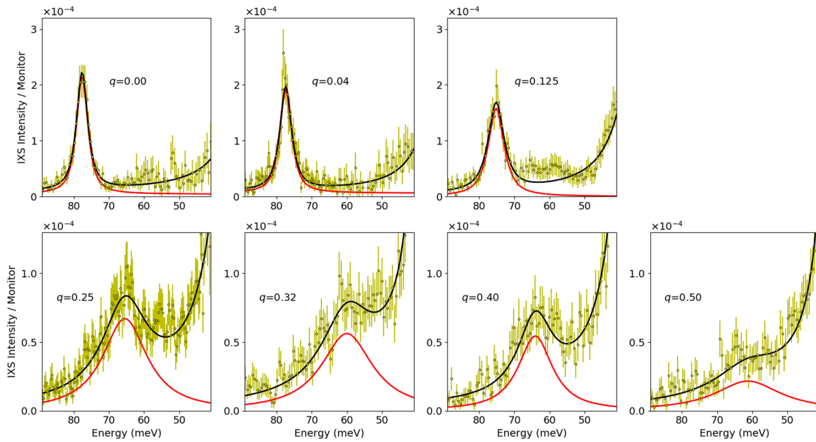
FIG. 4. Fits of the IXS spectra measured at 25 K at the ID28 beamline of ESRF in Na-CCOC plotted over the Cu-O bond-stretching phonon energy region demonstrating the quality of the fits. Pseudo-Voigt line shapes were used to fit the BS phonon mode. The data are shown with markers and the resulting fits are displayed with black-solid lines. The fitted BS phonons are highlighted with red lines. Normalized intensity corresponds to the ratio of IXS intensity with the beam monitor.
