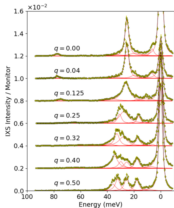
FIG. 9. IXS spectra measured for different Q = (3 - q, 0, 0) and at 25 K in Na-CCOC sample 2. The data have been recorded on the ID28 beamline of ESRF. The intensity for each wave vector below q = 0.5 are shifted of 0.2 \times 10^{-2} , so that the Brillouin zone center is at the top, and the zone boundary at the bottom. Figure 4 in the main text show a zoom of the same data, focusing on the details around the Cu-O bond-stretching mode energy range.
