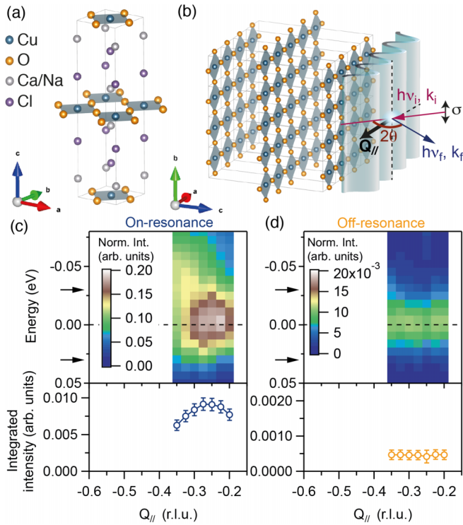
FIG. 1. (a) Crystal structure of Na-CCOC [25]. a , b , and c are the lattice axes of the sample. Cl ions are located on the apical sites. The four surrounding O form the square coordination of Cu, which is highlighted in blue. (b) Sketch of the RIXS scattering geometry with respect to the crystal structure of Na-CCOC and with a CDW. [(c),(d)] RIXS intensity maps recorded on- (c) and off- (d) resonance (top panels) as function of the energy and Q_{||} . The integrated intensities in the quasi-elastic regions (indicated with black arrows on the RIXS intensity maps) are plotted on the bottom panels.
