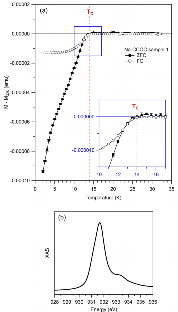
FIG. 7. (a) Zero-field-cooling (ZFC) and field-cooling (FC) magnetization measurements vs temperature with a magnetic field of 46.3 Oe of the Na-CCOC sample 1 (sample measured with RIXS) across the superconducting transition. The T_c corresponds to the onset of the diamagnetic signal. Inset shows an enlarged view of the signal within the blue box near T_c . (b) X-ray absorption spectrum (XAS) near the Cu L_3 -edge of Na-CCOC.
