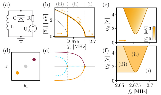
FIG. 5. Characterization of a single parametron. (a) Schematic of a parametron realization in the form of an RLC circuit with resistance R , inductance L , nonlinear capacitance C , and tuning voltage U_1 . (b) Amplitude response X_1 (orange lines) of the parametric resonator measured with a lock-in amplifier as a function of frequency f_d at a driving strength of U_d = 3 V. Arrows indicate the sweep direction. Thin gray solid (dashed) lines are calculated stable (unstable) steady-state solutions using the rotating steady states of Eq. (1) [cf. Eqs. (2)] with \lambda_1 = \frac{U_d}{U_{\text{th}}} \frac{2}{Q} = 0.017 , and \alpha_1 = -9 \times 10^{-17} \text{ V}^{-2} \text{ s}^{-2} used as a fit parameter [13]. (c) X_1 measured as a function of U_d and f_d using upsweeps (arrow) at constant U_d , showing a typical parametric instability lobe. The solid line is a theory fit to the lobe boundaries that allows for estimation of Q = 295 . (d) Schematic representation in phase space of the parametron phase states (wine red, orange), and the 0-amplitude state (gray). (e) Schematic representation of the steady-state solutions and bifurcation points as a function of f_d . Solid (dashed) lines indicate stable (unstable) solutions. (f) Calculated stability phase diagram. (i) White: only the 0-amplitude solution is stable; (ii) orange: only the phase states are stable; (iii) light orange: 0-amplitude and phase states are both stable. The regions (i)–(iii) manifest in (b) and (e).
