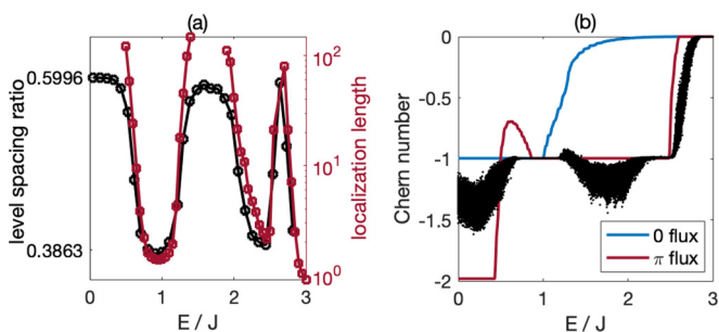
FIG. 5. (a) The left axis shows the level spacing ratio, for system size L_x = L_y = 60 with 10 000 disorder samples. The characteristic value for the Poisson ensemble, 2 \ln 2 - 1 \simeq 0.3863 , and the one for the Gaussian unitary ensemble, approximately equal to 0.5996, are indicated. The right axis shows the localization length obtained by one-parameter scaling for a sequence of quasi-1D long stripes for L_y = 8, 16, 32, 64, 128 and L_x \leq 10^6 . (b) Chern number for system size L_x = L_y = 40 . Black dots are for 500 disorder samples, while the blue (red) line is for the zero ( \pi ) flux clean system.
