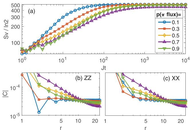
FIG. 4. Tuning the density of \pi fluxes. (a) Projective bipartite entanglement entropy of Majorana fermions. (b) and (c) Steady-state spatial correlation function |C^{zz(xx)}| , averaged in the time window 10^3 \lesssim Jt \lesssim 10^4 . The parameters are J_z = J_x = J_y \equiv J , \hbar = 0.25J , L_x = L_y = 50 , and 1000 disorder samples have been used.
