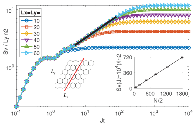
FIG. 3. Projective bipartite entanglement entropy, averaged over 1000 disorder samples. The inset shows the entanglement cut. The black line indicates the power-law fitting proportional to t^{1/z} with z = 2.4(1) . At late time, entropy saturates to a volume law S_v(Jt = 10^4) = 0.40(1)N \ln 2/2 , as shown in the inset.
