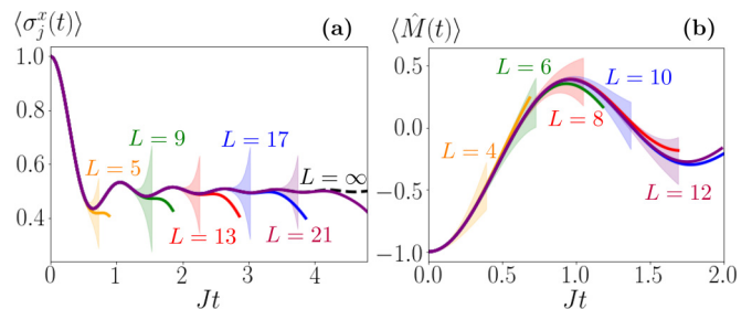
FIG. 2. Numerically exact evolution for (a) \langle\hat{\sigma}_j^x(t)\rangle in the L -site PBC TFIM at J = h , with |\psi(0)\rangle = |\rightarrow\rightarrow\dots\rangle , and (b) \langle\hat{M}(t)\rangle in the L -site OBC FHM at U = 0.5J , with |\psi(0)\rangle = |202020\dots20\rangle . The dashed curve in TFIM is the exact L \rightarrow \infty result. The shaded areas for each curve represent the region in which the actual L \rightarrow \infty values must lie according to the FSE bounds in Eqs. (11), (4), and (S19), respectively, and we do not show the shade beyond the timescale t_c \approx L/(2v) at which the error bounds become too large to be useful.
