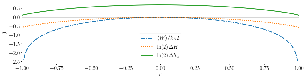
FIG. 5. Asymptotic work production \langle W \rangle , single-symbol \Delta H_1 bound, and Kolmogorov-Sinai-Shannon \Delta h_\mu bound when ratchet is driven by period-2 memoryful input. Since the input has no parameters, the parameter sweeps only over \epsilon with \tau = 10 .
