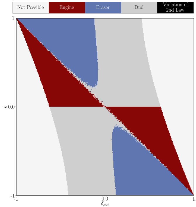
FIG. 10. Functional thermodynamic regions of a ratchet pattern deconstructor with an interaction interval of \tau = 0.75 . The x axis sweeps over the output bias \delta_{out} , while the y axis sweeps over \epsilon . As indicated, there are two parameter regimes where the ratchet is unable to act as a pattern deconstructor. In these regions, the desired output bias is not reachable by the machine at the given \epsilon . As \tau \rightarrow \infty , this region grows, until it encompasses every parameter combination other than \epsilon = \delta_{out} , which is always reachable with an input biased coin with bias \delta_{in} = \delta_{out} = \epsilon .
