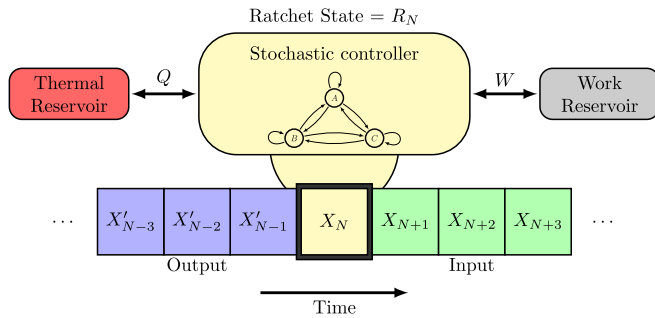
FIG. 1. Information engine as a finite-state ratchet (controller) connected to a thermal reservoir, a work reservoir, and an information reservoir (depicted as tape whose storage cells may be read or written).
