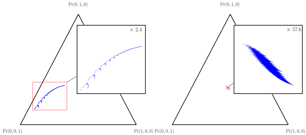
FIG. 4. Mixed states \eta \in \mathcal{R} of the output process generated by the ratchet driven with memoryless input [Fig. 2 (top row)] plotted on the 2-simplex. Corner labels give the mixed-state probability distributions \eta = (\text{Pr}(A \otimes D), \text{Pr}(B \otimes D), \text{Pr}(C \otimes D)) . Mixed states at the simplex corners correspond to the HMM being in exactly one of its states, while mixed states in the simplex interior are mixtures of the possible HMM states, with \eta = (\frac{1}{3}, \frac{1}{3}, \frac{1}{3}) lying at the center. (Left) Ratchet parameters \delta = -0.98, \epsilon = 0.01 , and \tau = 0.1 . (Right) Ratchet parameters \delta = 0.4, \epsilon = 0.5 , and \tau = 0.1 . Insets: detail of the mixed-state sets, magnified by amount indicated in upper right corner.
