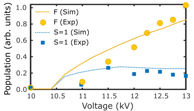
FIG. 4. Comparisons of decelerated populations between the F mode and S=1 mode at different applied voltages with a final velocity of 50 m/s. The points represent experimental results, while the lines are calculated via Monte Carlo simulation. Instead of showing saturation behavior as S=1 , the decelerated population using the F mode increases with higher applied voltage.
