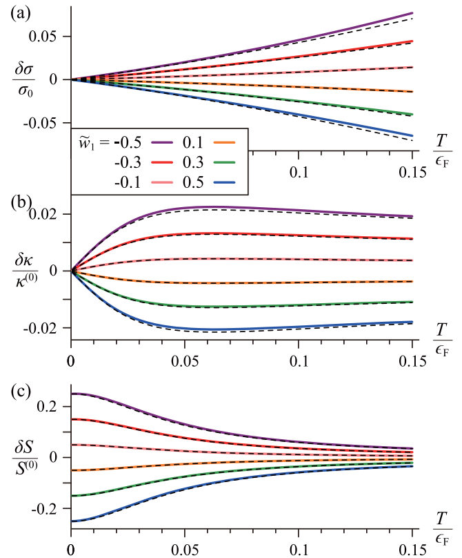
FIG. 6. The counterpart of Figs. 5(a)–5(c) for the nonanalytic form \delta\Gamma_{\mathbf{p}} = \tilde{w}_1 \gamma_{ei} \Theta(\xi_{\mathbf{p}}) \xi_{\mathbf{p}}/\epsilon_F of the elastic scattering rate.
