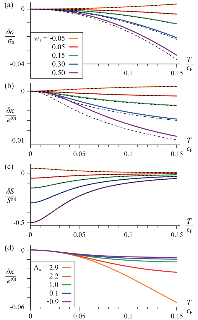
FIG. 5. The relative deviations of the electric conductivity \delta\sigma/\sigma^{(0)} (a), thermal conductivity \delta\kappa/\kappa^{(0)} (b), and Seebeck coefficient \delta S/S^{(0)} (c) caused by a momentum-dependent elastic scattering rate 1/\tau_{ei,\mathbf{p}} = \gamma_{ei} + \delta\Gamma_{\mathbf{p}} where \delta\Gamma_{\mathbf{p}} = w_1 \gamma_{ei} \xi_{\mathbf{p}}/\epsilon_F . All the curves were calculated within the RTA, with the relaxation rate matched to the one for two-dimensional Coulomb interactions (Sec. VA). Each curve corresponds to a different value of w_1 , and \gamma_{ei}/\epsilon_F = 0.01 . The dashed black lines show the results of the perturbative expansion with respect to w_1 . In (d) we present the relative deviation of the thermal conductivity for Fermi-liquid interactions in three dimensions with various values of \Lambda_a and fixed u = 1.29 [Eq. (32)] as well as w_1 = 0.5 .
