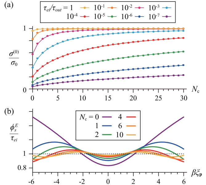
FIG. 8. (a) Convergence of the electric conductivity \sigma^{(0)}/\sigma_0 [Eq. (C21)] as a function of the cutoff N_c . Here, different values of \tau_{ei}/\tau_{out} are assigned to each solid line. (b) Plot for \phi_s^E(x)/\tau_{ei} as a function of x = \beta\xi_p . Here, different values of N_c are assigned to each solid line for fixed \tau_{ei}/\tau_{out} = 0.5 . The black dotted line is the guideline for the solution in the RTA [Eq. (14)].
