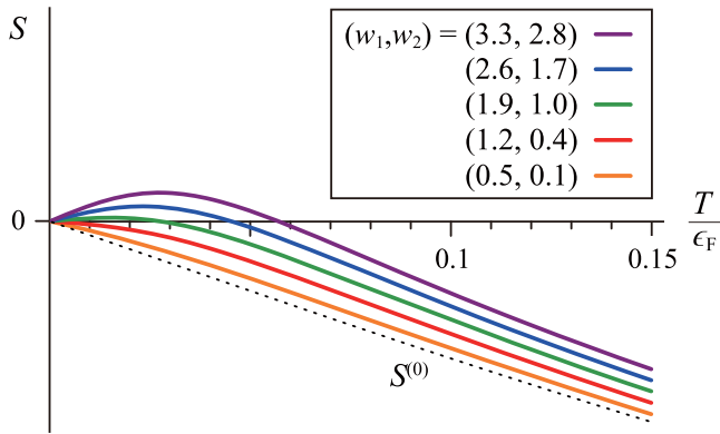
FIG. 7. The Seebeck coefficient in arbitrary units as a function of T/\epsilon_F . All curves were obtained by treating the electron-electron collision integral within the RTA and taking the momentum-dependent part of the electron-impurity scattering rate to be of the form \delta\Gamma_{\mathbf{p}}/\gamma_{ei} = w_1\xi_{\mathbf{p}}/\epsilon_F + w_2(\xi_{\mathbf{p}}/\epsilon_F)^2 . Different values of w_1 and w_2 lead to the solid lines for fixed \gamma_{ei}/\epsilon_F = 0.01 and u = 1.29 . The dotted black line represents S^{(0)} for the same value of \gamma_{ei}/\epsilon_F . A sign change of S occurs for w_1 > 1.5 .
