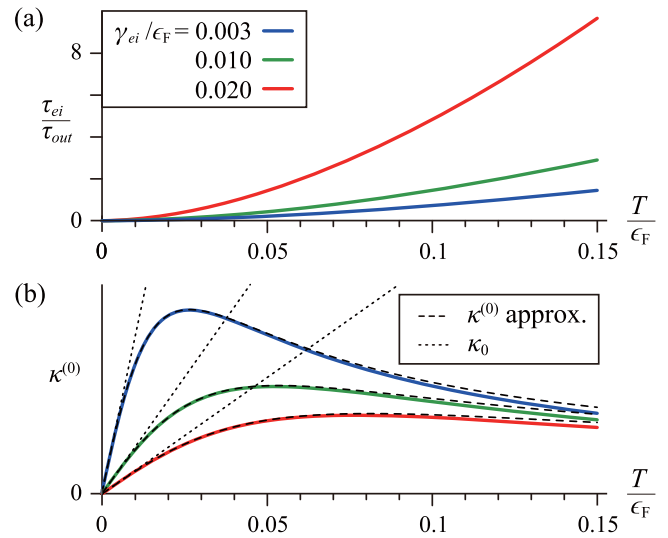
FIG. 3. Temperature dependence of \tau_{ei}/\tau_{\text{out}} at the Fermi energy \epsilon_F (a), and the thermal conductivity \kappa^{(0)} (b). The latter is shown in arbitrary units. All curves were obtained treating the electron-electron collision integral within the RTA in two dimensions. Each line corresponds to different values of \gamma_{ei} = \tau_{ei}^{-1} . In (b), the solid lines represent the full solution, while the dashed black lines were obtained through a perturbative expansion in T/\epsilon_F . The dotted black lines show \kappa_0 for the same values of \tau_{ei} .
