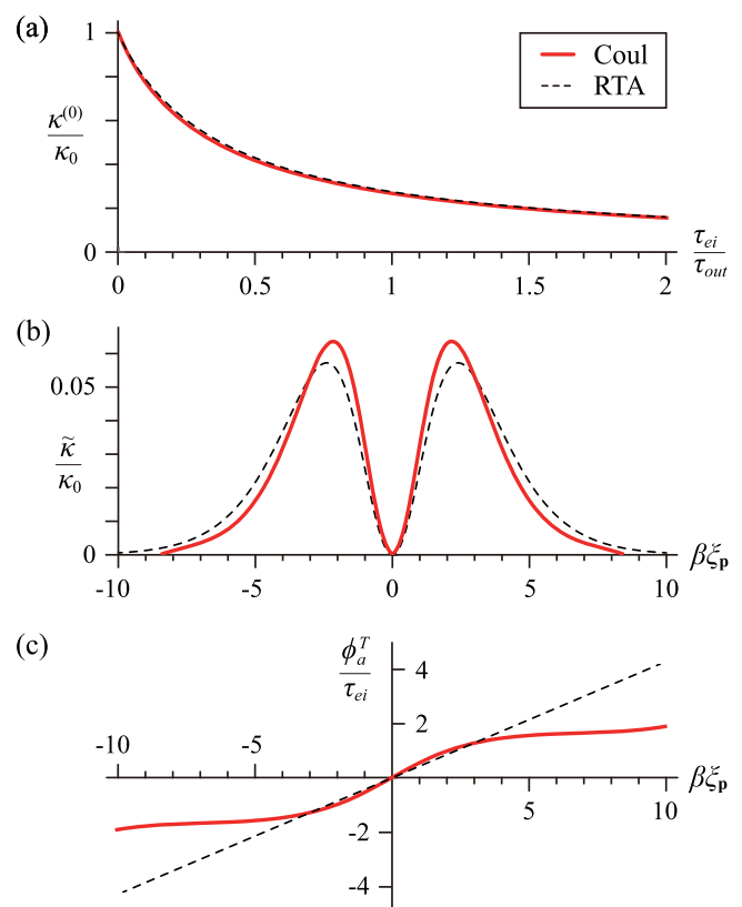
FIG. 1. (a) Thermal conductivity \kappa^{(0)} measured in units of \kappa_0 = \pi^2 \mathcal{N} T \tau_{ei} / (3m) as a function of \tau_{ei}/\tau_{\text{out}} . The curves were produced by solving the Boltzmann equation with the eigenfunction-expansion approach for Coulomb interactions in two dimensions (solid line), and using Keyes method within the RTA (dashed line). The inelastic relaxation time \tau_{ee} was chosen such that both results match in the clean limit (see discussion in Sec. V A). In (b) and (c), we plot the corresponding \tilde{\kappa}(x)/\kappa_0 and \phi_a^T(x)/\tau_{ei} , where x = \beta\xi_{\mathbf{p}} . \tilde{\kappa}(x) encodes the contribution from different energy shells. Here, we set \tau_{ei}/\tau_{\text{out}} = 0.5 .
