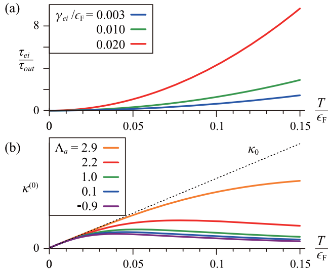
FIG. 4. The counterpart to Fig. 3 for FL interactions in three dimensions, with u = 1.29 . In (b) we fix \gamma_{ei}/\epsilon_F = 0.01 and look at different values of \Lambda_a .
