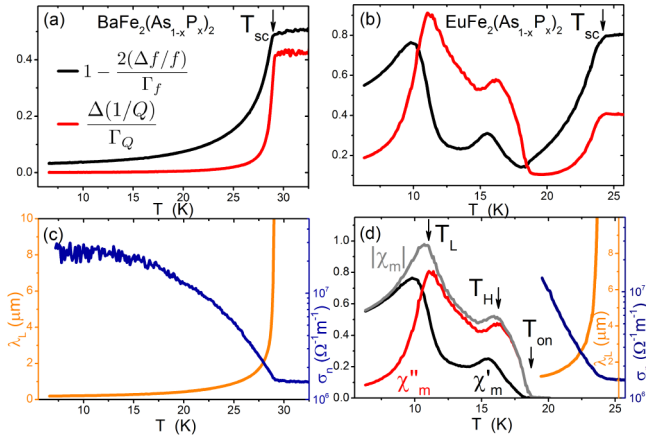
FIG. 2. Comparison between the microwave responses of \text{BaFe}_2(\text{As}_{1-x}\text{P}_x)_2 [(a), (c)] and \text{EuFe}_2(\text{As}_{1-x}\text{P}_x)_2 [(b), (d)]. In panels (a) and (b), black and red lines represent [1 - 2(\Delta f/f)/\Gamma_f] and \Delta(1/Q)/\Gamma_Q , respectively, where \Delta f and \Delta(1/Q) are the modifications in the resonance frequency and quality factor of a CPWR, induced by the crystal under study ( \Gamma_f and \Gamma_Q are geometrical factors). The arrows indicate the superconductivity onset temperature, T_{sc} . Panel (c) shows the London penetration depth, \lambda_L , and the quasiparticle conductivity, \sigma_n , as a function of temperature, obtained by the procedure described in the text from the data reported in panel (a). The same is reported in panel (d) for the data shown in panel (b), between T_{sc} and the onset of the magnetic signal, T_{on} (orange and blue curves and scales). At lower temperatures, a smooth baseline due to Meissner diamagnetism was subtracted from data in panel (b), and the real part \chi'_m , the imaginary part \chi''_m , and the modulus |\chi_m| of the bulk magnetic susceptibility were extracted according to the procedure described in the text [panel (d), black, red, and gray curves, left scale]. Other arrows indicate reference temperatures discussed in the text.
