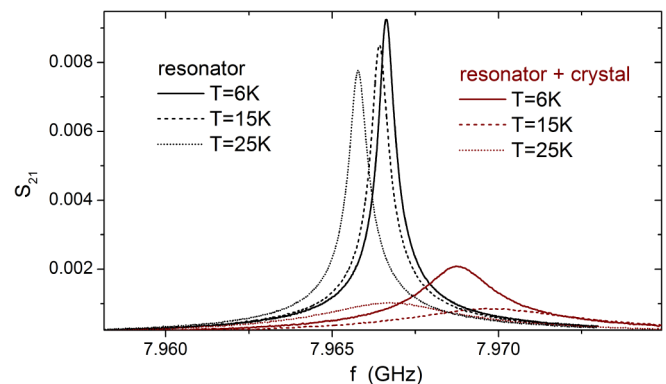
FIG. 6. Examples of resonance curves for the empty resonator and for the resonator with the crystal coupled to it.
