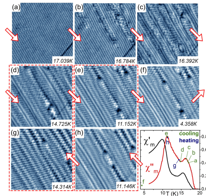
FIG. 5. MFM maps acquired on a x = 0.20 crystal at temperatures below T_{sc} and their link to peaks observed in microwave data. The maps reveal spatial variations of the out-of-plane component of the local magnetic field. Maps [(a)–(f)] correspond to the sample cooling [(f), (h), (g)] to heating. (a) Below Curie temperature, linear ferromagnetic Meissner domains form a short-period quasi-1D pattern. [(b)–(d)] Transition from DMS to DVS, between 16.8 K and 15 K, is characterized by the proliferation of DVS domains of a larger period and a more complex 2D organization. [(d), (g), (e), (h)] A hysteretic behavior is observed in maps acquired around 8–15 K upon temperature cycling (red dashed lines delimit pairs of maps acquired at close temperatures). (f) Below 8 K the DVS pattern is “frozen.”
