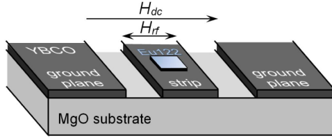
FIG. 7. Experimental configuration (not to scale).
