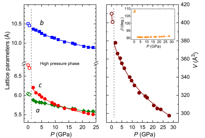
FIG. 3. The lattice parameters, unit-cell volume, and monoclinic angle (inset) of \text{MnPS}_3 as a function of pressure. The solid lines represent the fits based on the Birch-Murnaghan equation of state for the high-pressure phase.
