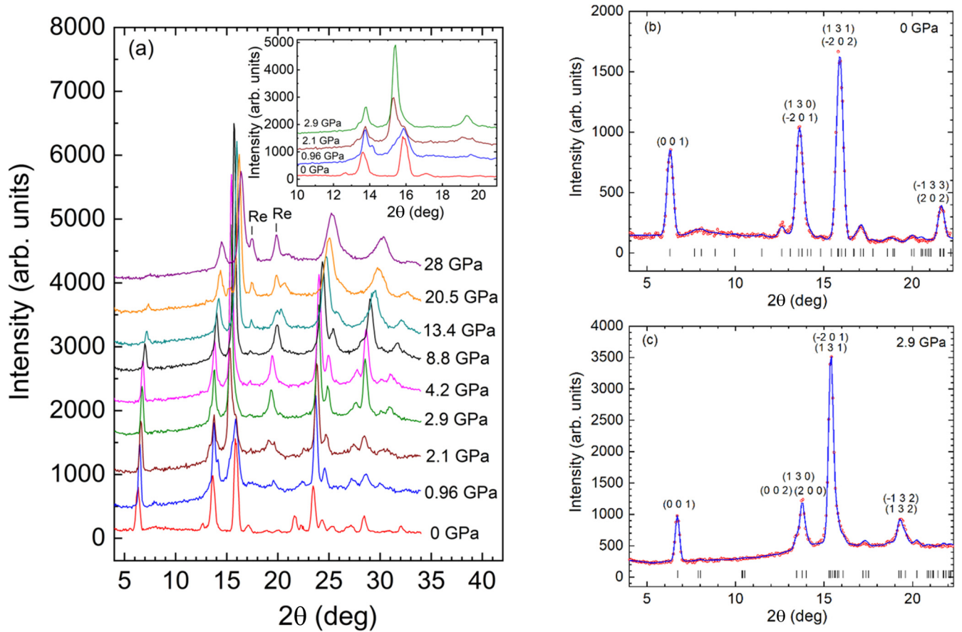
FIG. 2. XRD patterns of \text{MnPS}_3 , measured at selected pressures (a). The inset shows the evolution of enlarged parts of XRD patterns over the structural phase transition. Sections of XRD patterns, measured at ambient pressure (b) and P = 2.9 GPa (c), refined by the Rietveld method. The experimental curves and calculated profiles are shown. The ticks below represent the calculated positions of the diffraction peaks.
