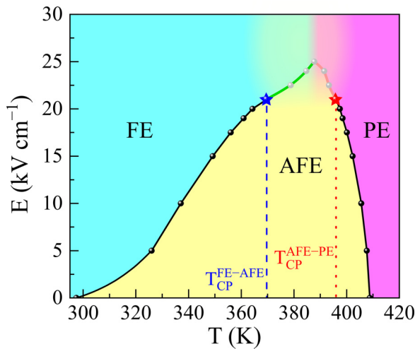
FIG. 3. Electric field–temperature phase diagram of antiferroelectric PNZST ceramics. Solid lines represent first-order FE-AFE and AFE-PE transition lines, which are terminated by critical end points marked with stars. Above critical end points, both transitions exhibit supercritical behavior. FE-AFE and AFE-PE phase transitions merge at 25 \text{ kV cm}^{-1} and 387.8 \text{ K} .
