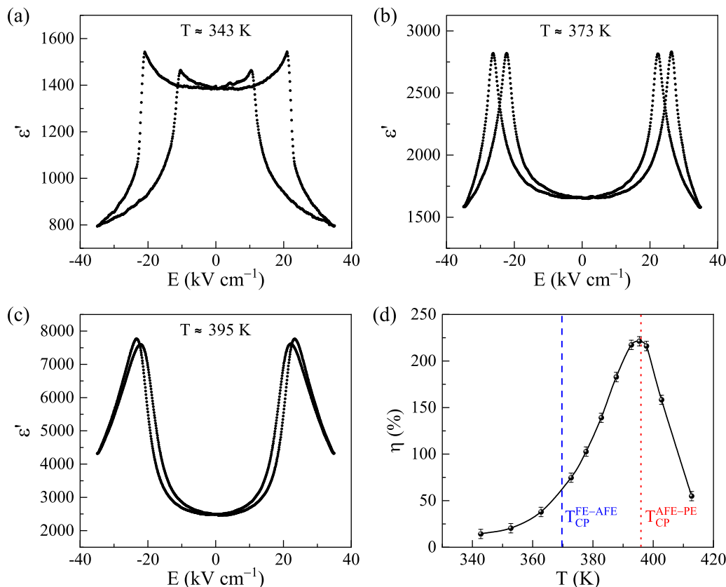
FIG. 4. (a), (b), and (c) Evolution of dielectric permittivity as function of electric field during second measurement loop in PNZST at representative temperatures involving first-order AFE-FE phase transition, FE-AFE critical end point, and AFE-PE critical end point, respectively. (d) Tunability of dielectric response as function of temperature. Dashed and dotted lines represent temperatures of FE-AFE and AFE-PE critical end points, respectively.
