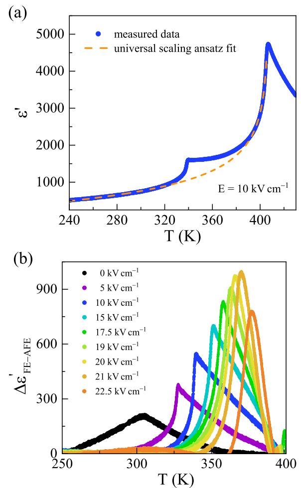
FIG. 2. (a) Dielectric response measured at 10 \text{ kV cm}^{-1} . Dashed line represents fit to universal scaling ansatz. (b) Dielectric anomaly of dielectric permittivity around FE-AFE phase transition, after fitted background was subtracted from measured data. Maximum dielectric response of FE-AFE phase transition is determined at 21 \text{ kV cm}^{-1} and 369.7 \text{ K} .
