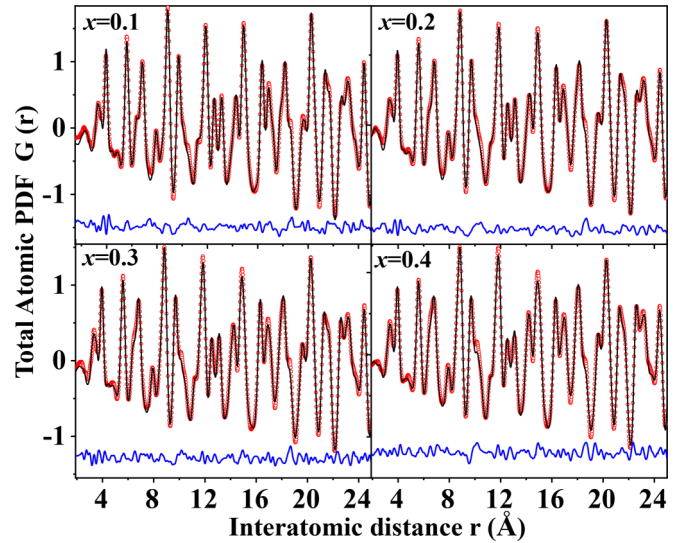
FIG. 5. Crystallographic (small unit cell) fits (black) to experimental PDFs G(r) (red) for La substituted \text{Bi}_{1-x}\text{La}_x\text{FeO}_3 based on a S.G. P1 model. The residual difference (blue) is shifted by subtracting a constant for clarity. The goodness-of-fit indicator, R_{\text{wp}} , for the fits is about 13%.
