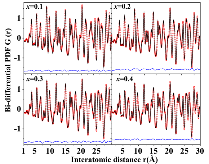
FIG. 7. RMC (large model based) fits (black) to experimental Bi-differential PDFs G(r) (red) for La substituted \text{Bi}_{1-x}\text{La}_x\text{FeO}_3 . The initial configuration is based on a S.G. P1 type structure. The residual difference (blue) is shifted by subtracting a constant for clarity. The goodness-of-fit indicator, R_{\text{wp}} , for the fits is about 6%.
