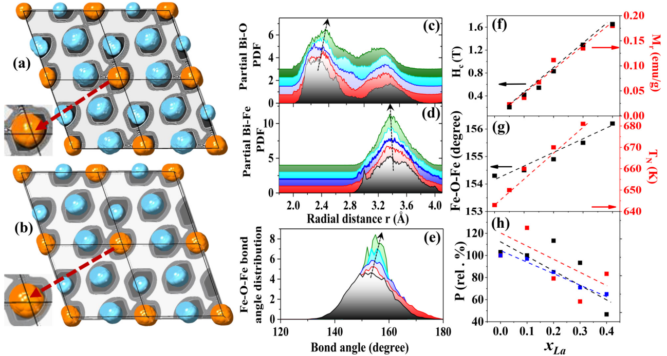
FIG. 8. Projection of the RMC refined model for (a) BiFeO 3 and (b) Bi 0.6 La 0.4 FeO 3 onto the (001) R atomic plane of the perovskite lattice. For simplicity, Fe atoms are not shown. Bi atoms are in brown and oxygen atoms are in blue. The gray shaded contour boundaries include 99% of all atoms at the particular lattice sites. The blue/orange-colored regions include all atoms at the particular site, where atoms that are closer than 0.5 Å are merged. Bi atoms in Bi 0.6 La 0.4 FeO 3 appear less displaced from the geometrical centers of the oxygen polyhedron that encloses them in comparison to a Bi atom in pure BFO (compare the positions of the crosshair type projection of the unit cell edges on the distribution of Bi atoms at the center of the plots, which, for clarity, is also shown enlarged on their left side). Partial (c) Bi-O and (d) Bi-Fe PDFs G(r) computed from the RMC refined models for Bi 1-x La x FeO 3 ( x = 0, 0.1, 0.2, 0.3, \text{ and } 0.4 ). (e) Distribution of Fe-O-Fe bond angles computed from the RMC models; (f) our experimental data for the coercive field H_c and remanent magnetization M_r for pure and La substituted BFO. (g) RMC model averaged Fe-O-Fe bond angles (black) and experimental Néel temperature T_N (red) for La substituted BFO. (h) Change in computed spontaneous (blue) and experimental saturation (red) and remanent (black) polarization in La substituted BFO. Broken lines in (f)–(h) are a guide to the eye. Arrows in (c)–(e) highlight trends in the shown data sets with increasing La content x_{La} from x = 0 (black) to x = 0.4 (green).
