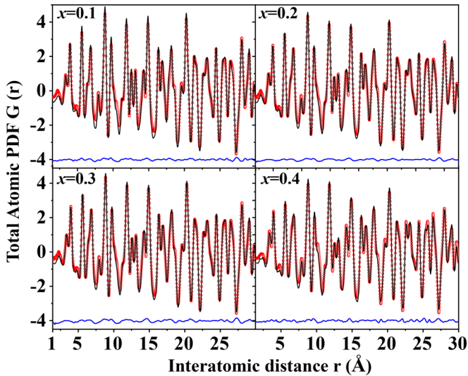
FIG. 6. RMC (large model based) fits (black) to experimental PDFs G(r) (red) for La substituted \text{Bi}_{1-x}\text{La}_x\text{FeO}_3 . The initial configuration is based on a S.G. P1 type structure. The residual difference (blue) is shifted by subtracting a constant for clarity. The goodness-of-fit indicator, R_{\text{wp}} , for the fits is about 6%.
