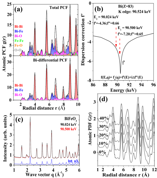
FIG. 2. (a) Computed total and Bi-differential atomic pair correlation functions (PCFs) g(r) (black) for pure \text{BiFeO}_3 . The individual partial PCFs are also shown, each in a different color. (b) Energy dependence of the real dispersion correction f' for Bi. The energies below the K edge of Bi used in the present experiments are marked with arrows. Values for f' and f'' at these energies are also given. (c) XRD patterns for \text{BiFeO}_3 taken at 25 eV (red) and 500 eV (black) below the K edge of Bi (90.524 keV). Their difference (blue) multiplied by a factor of 3 is also given. (d) Experimental Bi-differential atomic PDFs G(r) for pure and La substituted \text{BiFeO}_3 . The PDFs are offset vertically for clarity. Note that, as defined, the PCF g(r) = \rho(r)/\rho_0 , oscillates about 1 while the PDF G(r) = 4\pi r \rho_0 [\rho(r) - 1] oscillates about zero. Here \rho(r) and \rho_0 are the local and average atomic number density, respectively.
