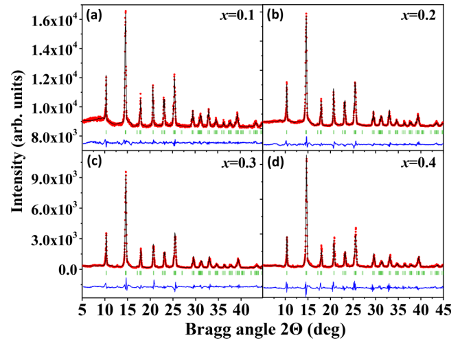
FIG. 3. Rietveld fits (black) to XRD patterns (red) for La substituted \text{Bi}_{1-x}\text{La}_x\text{FeO}_3 based on a S.G. R3c model. Vertical green bars show the position of Bragg peaks. The residual difference (blue) is shifted by subtracting a constant for clarity. The goodness-of-fit indicator, R_{\text{wp}} , is about 6% for the x = 0.1 and x = 0.2 samples. It is about 13% and 16% for the x = 0.3 and x = 0.4 samples, respectively.
