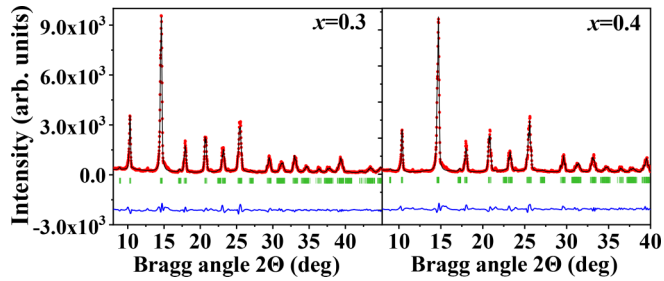
FIG. 4. Rietveld fits (black) to XRD patterns (red) for La substituted \text{Bi}_{1-x}\text{La}_x\text{FeO}_3 based on a S.G. P1 model. Vertical green bars show the position of Bragg peaks. The residual difference (blue) is shifted by subtracting a constant for clarity. The goodness-of-fit indicator, R_{\text{wp}} , is about 7% and 9% for the x = 0.3 and x = 0.4 samples, respectively.
