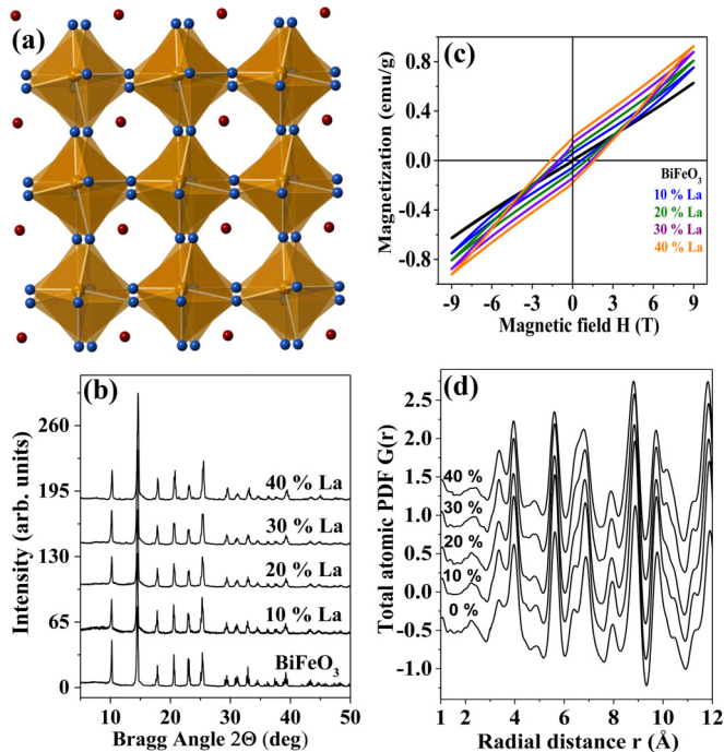
FIG. 1. (a) Fragment from the rhombohedral structure of \text{BiFeO}_3 projected down the \langle 001 \rangle_R direction, featuring corner shared Fe (brown circles)–oxygen (blue circles) octahedra with Bi (red circles) atoms positioned in the cavities between them. The octahedra are rotated with respect to each other and Bi atoms are displaced from the geometrical center of the cavities, rendering the material ferroelectric. (b) XRD patterns, (c) room temperature hysteresis curves, and (d) total atomic PDFs G(r) for pure and La substituted \text{BiFeO}_3 . The PDFs are offset vertically for clarity.
