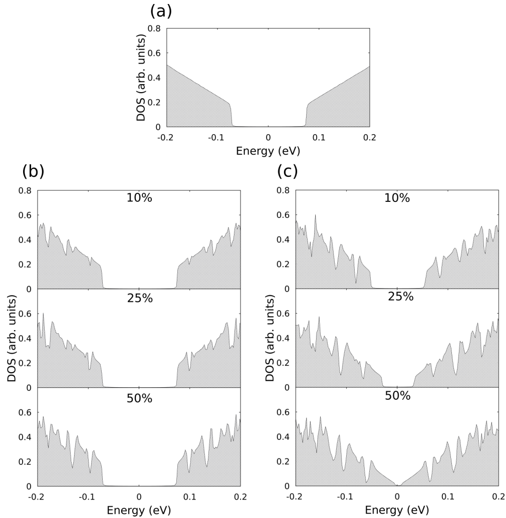
FIG. 6. Electronic density of states of (a) periodic, (b) location, and (c) rotation disordered models computed by tight-binding calculations. Each model has been built using the original 8 \times 8 cell containing a single borazine ring [see Fig. 1(a)]. Moreover, different disorder concentrations have been considered as indicated in each frame. Location disorder models have been built using the model M_2 described in the Supplemental Material. In (c), the rotation disorder is added in the location disordered system in (b) with 25% of displaced BN rings.
