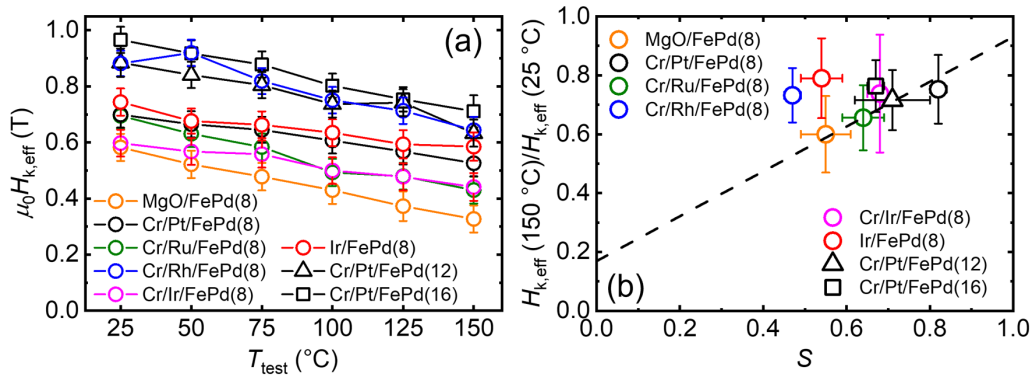
FIG. 3. (a) H_{k,\text{eff}} vs T_{\text{test}} for all FePd films deposited on different buffer layers. (b) The ratio of H_{k,\text{eff}} at 150 °C to its RT value as a function of S . The dashed line guides the general trend.
