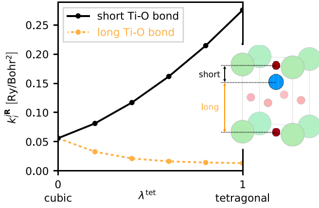
FIG. 6. Magnitude of interatomic forces k_i^{jR} between titanium and the nearest-neighbor apical oxygen atoms as a function of \lambda^{\text{tet}} (defined in Sec. IV). Solid black line corresponds to the Ti-O bond which shortens with \lambda^{\text{tet}} . Orange color corresponds to the elongated Ti-O bond. These bonds are also indicated in the inset. For \lambda^{\text{tet}} above roughly 0.5, the elongated bond is effectively broken as calculated k_i^{jR} tends to zero. Indices i , j , and lattice vector \mathbf{R} are selected so that the value of k_i^{jR} used in the plot corresponds to the pairs of nearest-neighbor Ti and apical O atoms.
