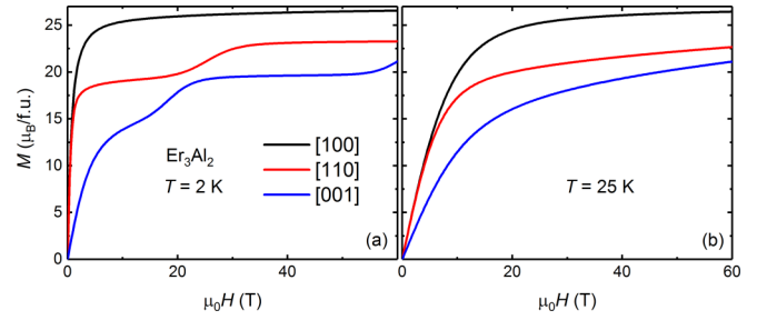
FIG. 5. Field dependences of the magnetization, M , at (a) 2 and (b) 25 K calculated for \text{Er}_3\text{Al}_2 using the CEF parameters listed in Table I.
