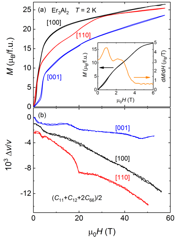
FIG. 2. Field dependences of (a) the magnetization, M , and (b) relative sound velocity, \Delta v/v , of longitudinal acoustic waves for field applied along the principal crystallographic directions of \text{Er}_3\text{Al}_2 at 2 K. The inset in (a) shows M and its field derivative, dM/dH , for field applied along the [100] axis up to 6 T. The ultrasound frequencies were 36, 42, and 82 MHz for field applied along the [100], [110], and [001] axes, respectively. In (b), the curves are vertically shifted for clarity.
