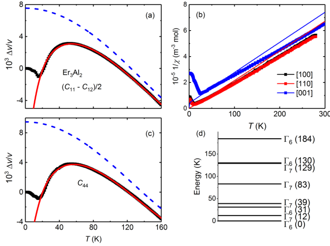
FIG. 4. Temperature dependences of (a) and (c) the relative sound-velocity, \Delta v/v , for the transverse acoustic modes (C_{11} - C_{12})/2 and C_{44} , respectively, and (b) the inverse magnetic susceptibility, 1/\chi . (d) CEF level scheme of an \text{Er}^{3+} ion in \text{Er}_3\text{Al}_2 obtained from the CEF parameters listed in Table I. In (a)–(c), the symbols and the solid lines represent the experimental and calculated data, respectively. The dashed lines in (a) and (c) represent the background stiffness. In (d), all horizontal lines correspond to doublets.
