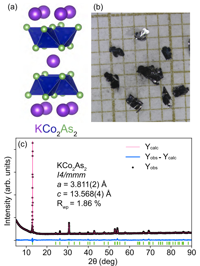
FIG. 1. (a) Crystal structure of \text{KCo}_2\text{As}_2 showing two-dimensional \text{CoAs} planes with \text{K}^+ ions between adjacent layers. (b) Representative shiny, silver, and thin crystals (on 1 \times 1 \text{ mm}^2 paper) grown with the discussed method after remaining flux had been removed by washing with anhydrous ethanol. (c) Powder x-ray diffraction patterns with \text{Cu K}\alpha radiation of \text{KCo}_2\text{As}_2 in the body-centered tetragonal structure ( I4/mmm ) at room temperature (about 295 K). Green tick marks representing the corresponding tetragonal phase are shown below the calculated, observed, and difference curves from Rietveld analysis.
