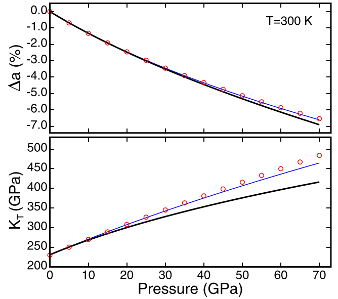
FIG. 5. Percent variation of the lattice parameter (top) and bulk modulus (bottom) of MgO at 300 K vs pressure calculated by using a conventional QHA approach (red circles) and the methods presented in this work (solid lines), i.e., explicit calculation by using our QHA method of thermal stress, and isochoric-isothermal linear and nonlinear elastic constants for a reference state yielding a zero static pressure, followed by the extrapolation procedures relying on nonlinear continuum mechanics described in Sec. IV. The black solid line shows results obtained by combining Eqs. (8) and (11), whereas the thin blue solid line shows results obtained by including in Eq. (8) also the leading third-order terms in strain [Eq. (29)], whose coefficients are the isothermal-isochoric fourth-order elastic constants C_{\alpha\beta\beta\beta}^{(4)} , with \alpha, \beta = 1, \dots, 6 .
