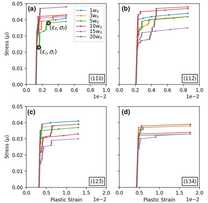
FIG. 7. [(a)–(d)] Several stress-strain curves from screw dislocation propagation simulations on each slip plane type. The curves show a characteristic “staircase” as dislocations are pinned and unpinned several times before finally annihilating with periodic images. The definitions of \sigma_i and \sigma_f are illustrated in panel (a).
