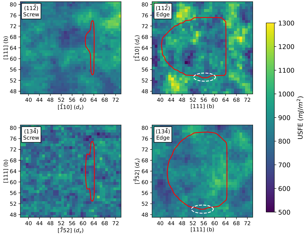
FIG. 4. The critical stages of FR source activation for both a plane with a low screw-edge ratio, \{112\} type, and a plane with a high screw-edge ratio, \{134\} type. Both screw- and edge-oriented sources show kink-pair nucleation as the limiting step. Before these kink pairs form, the dislocation will fall back to its original position if the stress is unloaded. The correlation lengths used in these examples range from 1w_0 to 10w_0 .
