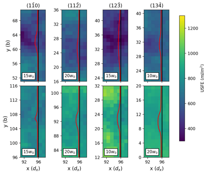
FIG. 12. Examples of kink-pair nucleation on all four slip planes. The kink pairs in the top row are nucleated on the weakest screw dislocation for their slip plane, while the bottom row shows kink pairs on the strongest screw dislocation studied. The black line shows the initial placement of the dislocation at zero stress. Regardless of the slip plane, correlation length l , or critical stress, kink-pair nucleation controls the glide behavior of the dislocations.
