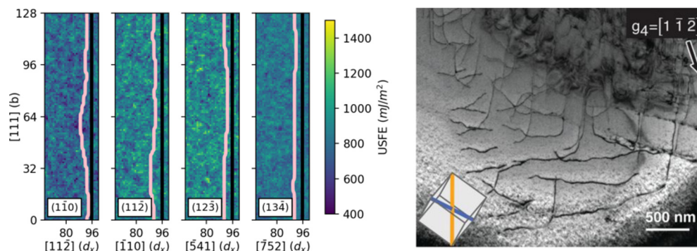
FIG. 11. (Left) Examples of dislocations that were unloaded during glide in PFDD. The black line is the initial dislocation and the pink line is the unloaded dislocation. Just as the dislocations are wavy during glide, they remain wavy under zero stress if the stress is removed. The correlation length l is 1w_0 for all four cases pictured. (Right) Experimental observations of wavy dislocations in MoNbTi. Taken with permission from Ref. [27].
