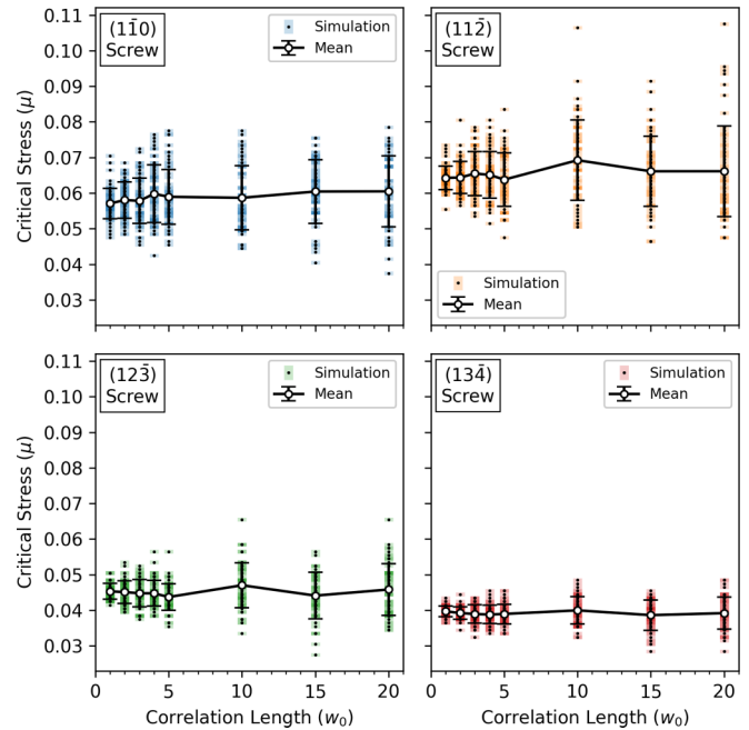
FIG. 3. The critical stresses to activate a screw-oriented FR source on each plane. Each colored box is a separate simulation, and darker colors indicate where multiple simulations give the same critical stress value. The mean for each correlation length is also plotted with error bars corresponding to the standard deviation of the distribution.
