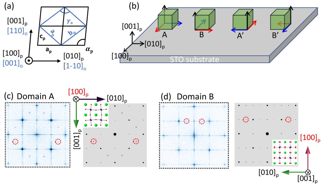
FIG. 5. (a) Distorted orthorhombic film on cubic substrate under compressive strain. “o” and “p” index refer to the orthorhombic and pseudocubic lattice parameters, respectively. (b) Four 90^\circ rotated domains are expected as shown. Red arrow points to the direction of in-phase rotation of the neighboring octahedra in Glazer notation. Two distinctly different domains are observed in STEM taken along [100] beam direction. (c) FFT of domain A and simulated diffraction obtained with the beam direction the same as the direction of in-phase rotation of the model structure (inset). (d) FFT of domain B and simulated diffraction with the beam direction perpendicular to the in-phase rotation axis.
