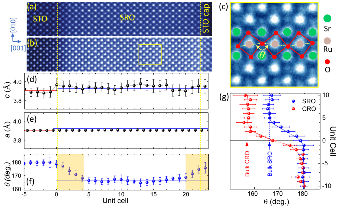
FIG. 4. Quantitative analysis of a 22-u.c. SRO film with STEM: (a) HAADF and (b) ABF images taken along the [100] direction of the substrate. (c) A zoom-in of a region of ABF image in (b) overlapped with schematic octahedral rotations. (d) The out-of-plane (OOP) and (e) in-plane (IP) lattice parameters extracted from the HAADF images. Both the substrate STO-film interface and the capping STO-film interface are shown as orange dashed lines. Red and blue lines mark the pseudo-cubic lattice parameters of the corresponding bulk structures, respectively. (f) The oxygen octahedral tilt angles extracted from the ABF image in (b) is plotted vs film thickness. The Ru-O-Ru bond angle of 180^\circ for STO (red line) and 166^\circ for bulk orthorhombic SRO (blue line) as well as the emphasized interface regions (shaded) are marked. (g) A comparison of octahedron tilts near interface of SRO/STO to CRO/STO.
