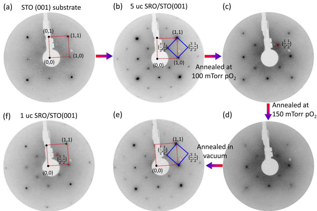
FIG. 2. LEED images taken at room temperature with a beam energy of 74 eV: (a) (1 \times 1) Bulk truncated STO (001) surface overlapped with a red square for surface unit cell. (b) A 5-u.c. SRO film on STO (001) showing (\sqrt{2} \times \sqrt{2})R45^\circ reconstructed unit cell (blue square) with respect to the substrate one. (c)–(e) The same sample under various annealing conditions. (f) A 1-u.c. SRO film.
