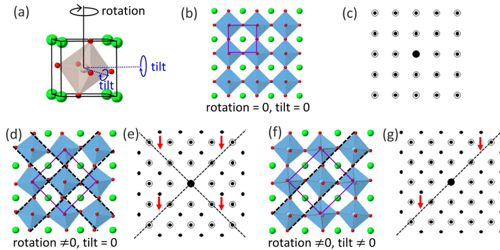
FIG. 3. Simulated LEED diffraction patterns for different surface symmetry. (a) A schematic showing \text{RuO}_6 tilt and rotations. (b), (c) Top view of a square lattice with no \text{RuO}_6 rotation or tilt and the corresponding diffraction pattern. The integer spots due to a square lattice are shown as a dot with a concentric circle. (d), (e) Square lattice where \text{RuO}_6 octahedra are rotated but not tilted and the corresponding diffraction pattern. Fractional spots are shown as solid dots. Glide lines are shown with dashed lines. Arrows indicate the position of missing fractional spots. (f), (g) Lattice with both \text{RuO}_6 tilts and rotation as well as the corresponding diffraction pattern. Only one glide line survives as shown with dashed lines.
