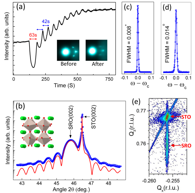
FIG. 1. (a) RHEED oscillations of the initial growth of SRO films on STO(001) surface. The inset shows the diffraction pattern before and after film growth. (b) Coupled x-ray diffraction scan of a \sim 47 -unit-cell thick SRO film. The Laue oscillations are fitted and presented in the red curve. Inset shows a schematic orthorhombic structure of bulk SRO. Panels (c) and (d) show rocking curves of the substrate and film peak, respectively. (e) Reciprocal space mapping about the (-103) Bragg diffraction spot. The substrate peak and the film peak are marked.
