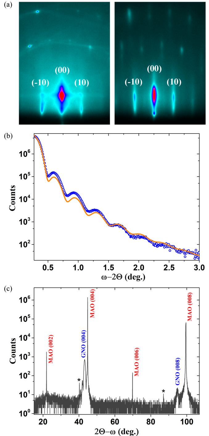
FIG. 2. Characterization of the grown GNO thin film. (a) On the left, the RHEED pattern of the (001)-oriented MAO substrate at 650^\circ\text{C} , and on the right, the RHEED pattern of the grown GNO film at room temperature. (b) The fit of the XRR curve for the same sample yields 11.79(4) \text{ nm} film thickness and 240(20) \text{ pm} surface roughness. (c) 2\Theta-\omega x-ray diffraction scan along the 00l direction. The scan contains allowed reflections of the substrate and fabricated film together with two forbidden reflections (002 and 006) of the substrate which arise because of the Umweganregung effect [31]. Asterisks mark (004) and (008) peaks of the substrate due to residual K_\beta radiation.
