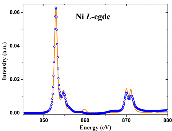
FIG. 4. Ni L -edge XAS spectrum of the GNO film. Blue dots are the measured data whereas the orange line shows the simulated spectrum of Ni 2+ .
