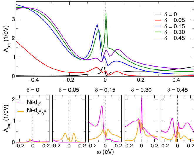
FIG. 7. Total spectral function after \mathbf{k} -integration (top) and local \text{Ni-}e_g spectrum (bottom) of pristine and hole-doped \text{NdNiO}_2 at low energy.
