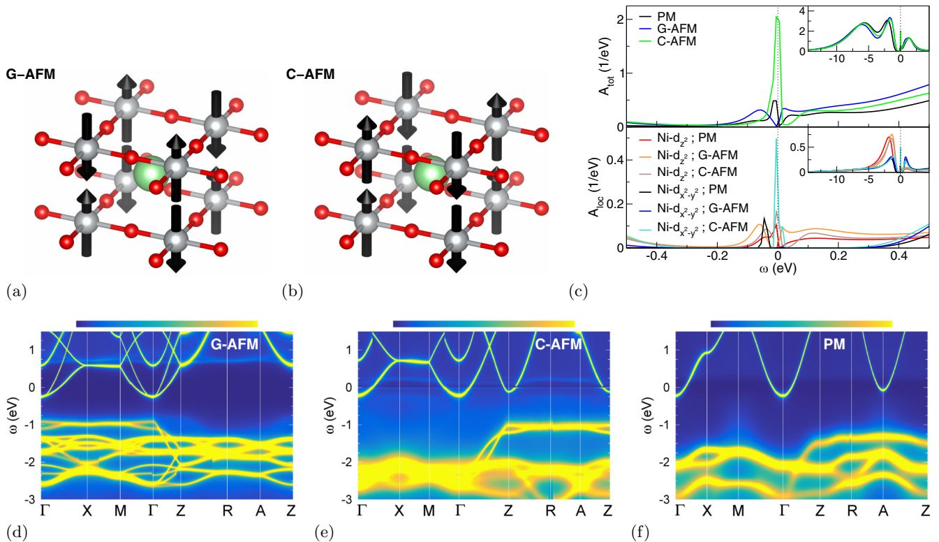
FIG. 8. Comparing PM and AFM-ordered \text{NdNiO}_2 . (a) G-AFM ordering and (b) C-AFM ordering. (c) Total (top) and local \text{Ni-}e_g (bottom) spectral function for PM, G-AFM and C-AFM phase, respectively. (d)–(f) \mathbf{k} -resolved spectral function along high symmetry lines for the (d) G-AFM, (e) C-AFM, and (f) PM phases. The \sqrt{2} \times \sqrt{2} enlarged in-plane unit cell translates into X \leftrightarrow M and R \leftrightarrow A for the (G,C)-AFM structure. And the upper \text{Ni-}d_{z^2} flat-band part is flipped with respect to k_z for the G-AFM structure due to the doubled unit cell along c .
