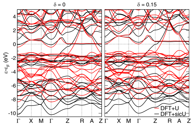
FIG. 12. Comparison between the DFT + U (red) and DFT + sicU band structure for pristine (left) and \delta = 0.15 hole-doped (right) NdNiO 2 in the C-AFM phase.
