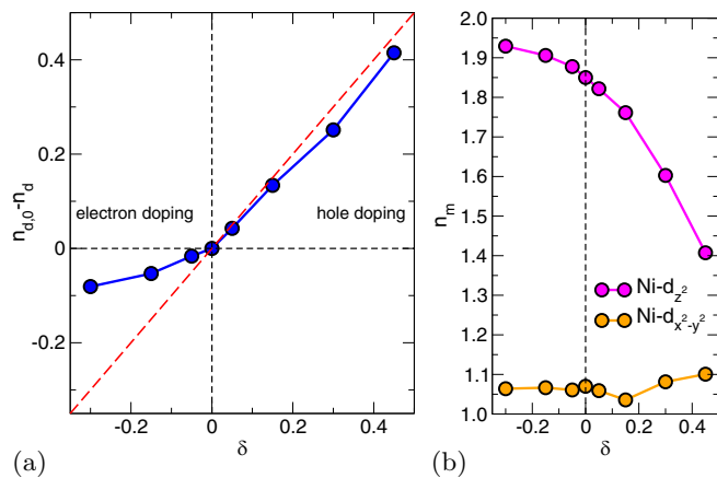
FIG. 3. Effective Ni(3d) occupation in doped NdNiO 2 from introducing \delta holes/electrons. (a) Difference n_{d,0} - n_d between the total occupation at n_{d,0} zero doping and at given doping n_d , versus \delta . The dashed red line marks the regime where the complete doping charge is transferred to Ni(3d). (b) Orbital-resolved filling of the Ni- e_g states.
