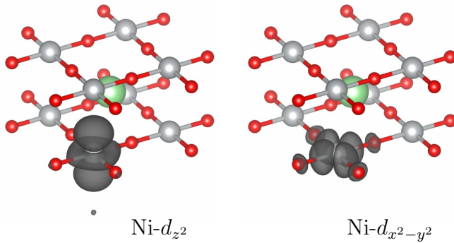
FIG. 1. Projected local orbitals of Ni- d_{z^2} (left) and Ni- d_{x^2-y^2} (right) type in the NdNiO 2 compound: Ni(grey), Nd(large,green), O(small,red).
