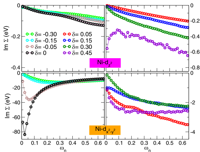
FIG. 5. Imaginary part \text{Im} \Sigma(i\omega_n) of the Ni- e_g self energy on the Matsubara axis \omega_n = (2n + 1)\pi T for different dopings \delta . Top: Ni- d_{z^2} and bottom: Ni- d_{x^2-y^2} . Left part: \delta = -0.30, -0.15, -0.05, 0 and right part: \delta = 0.05, 0.15, 0.30, 0.45 .
