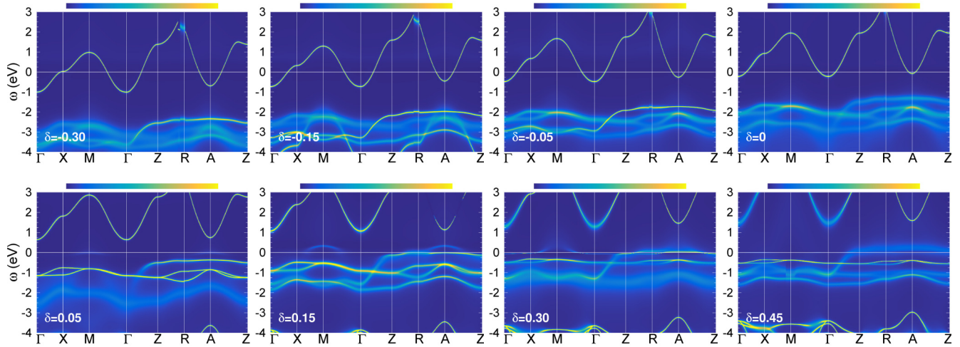
FIG. 4. Spectral function A(\mathbf{k}, \omega) with doping \delta . Top row, from left to right: \delta = -0.30, -0.15, -0.05, 0 . Bottom row, from left to right: \delta = 0.05, 0.15, 0.30, 0.45 . Same setting as in Fig. 2(a).
