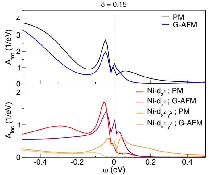
FIG. 9. Comparison of PM and G-AFM low-energy spectral functions at doping level \delta = 0.15 . (Top) Total spectrum and (bottom) local Ni- e_g spectrum.
