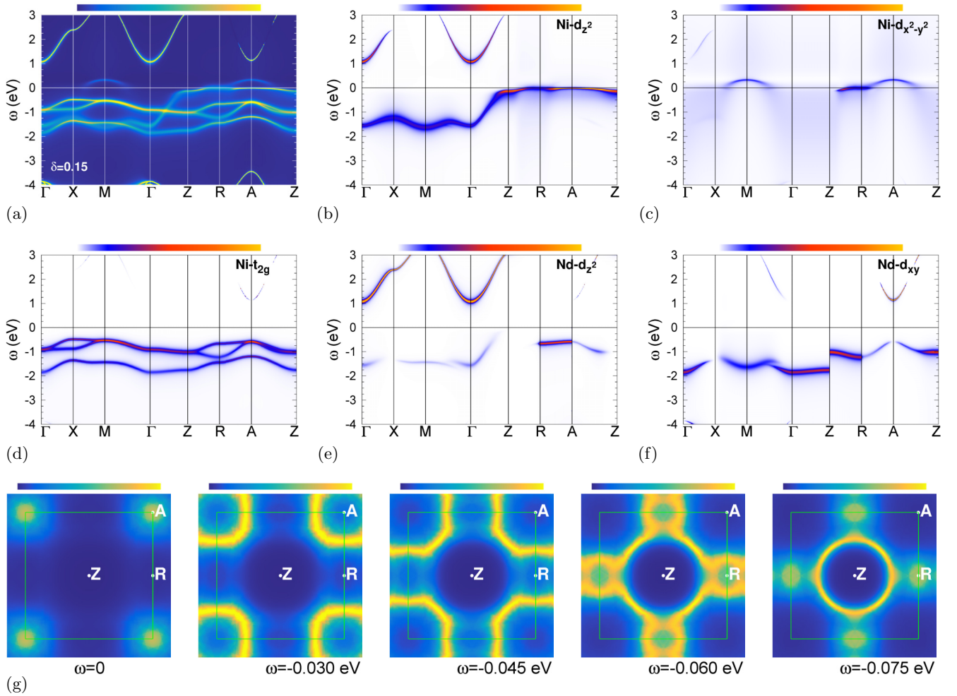
FIG. 6. Spectral information of hole-doped \text{NdNiO}_2 with \delta = 0.15 . (a)–(f) As in Figs. 2(a) to 2(f). (g) Constant-energy surfaces in the k_z = 1/2 plane. Note that the maximum intensity for the surfaces in (g) is reduced by a factor of 3 compared to the one for A(\mathbf{k}, \omega) in (a).
