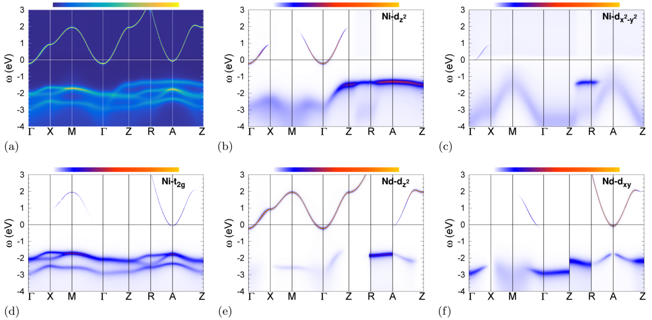
FIG. 2. Spectral information for pristine NdNiO 2 . (a) \mathbf{k} -resolved function A(\mathbf{k}, \omega) along high-symmetry lines: \Gamma -X-M describes a triangle in the k_z = 0 plane and Z-R-A marks the same triangle translated to the k_z = 1/2 plane. Above the Fermi level, only the single SD dispersion is shown and further dispersions discarded in the plot. (b)–(f) \mathbf{k} -resolved orbital weights (i.e., flat-bands) for the given spectral function: (b) Ni- d_{z^2} , (c) Ni- d_{x^2-y^2} , (d) Ni- t_{2g} , (e) Nd- d_{z^2} , and (f) Nd- d_{xy} . Note that with this chosen intensity resolution, the nondispersing-level feature at \varepsilon_F , giving rise to a Kondo(-lattice) mechanism [19] at lower T is not visible in A(\mathbf{k}, \omega) .
