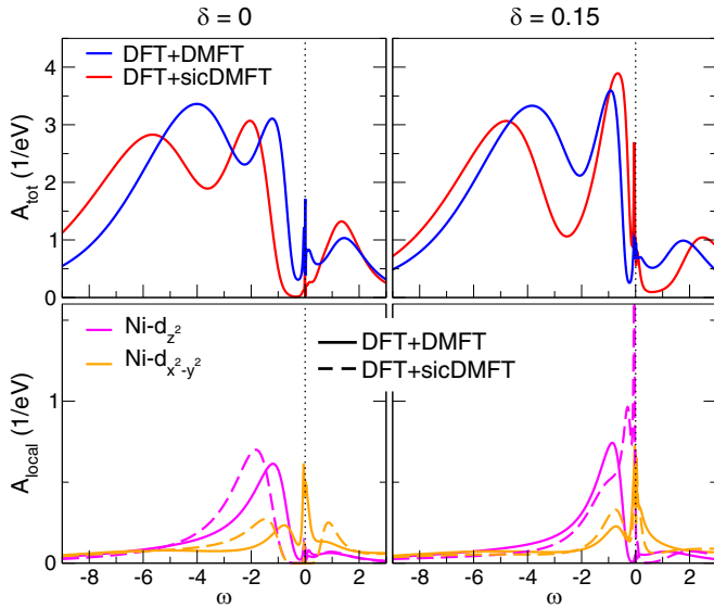
FIG. 10. Comparison of DFT + DMFT and DFT + sicDMFT spectral functions for pristine NdNiO 2 (left) and at doping level \delta = 0.15 (right). (Top) Total spectrum and (bottom) local Ni- e_g spectrum.
