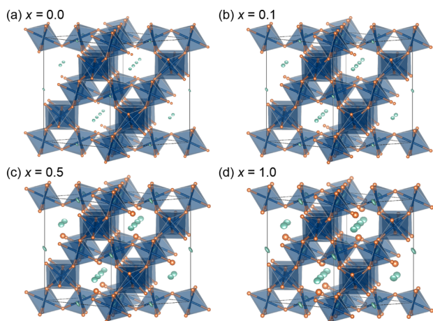
FIG. 5. Crystallographic structures for the series (Pr_{1-x}Bi_x)_2Ru_2O_7 [(a) x = 0.0 , (b) x = 0.1 , (c) x = 0.5 , and (d) x = 1.0 ] indicates anisotropic ADPs of the A-site cation (shown at 90% probability) increase with Bi concentration.
