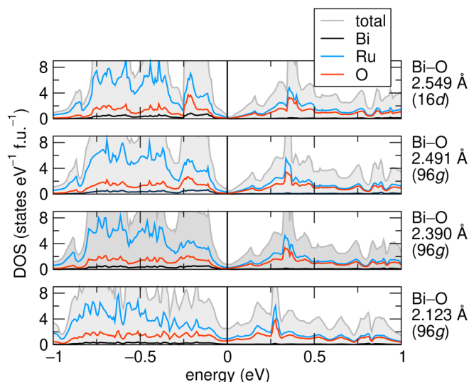
FIG. 10. Total and projected density of states (DOS) for stoichiometric Bi_2Ru_2O_7 as a function of the Bi^{3+} displacements from the 16d to 96g Wyckoff site. The energies are referenced to the Fermi at 0 eV (vertical line).
