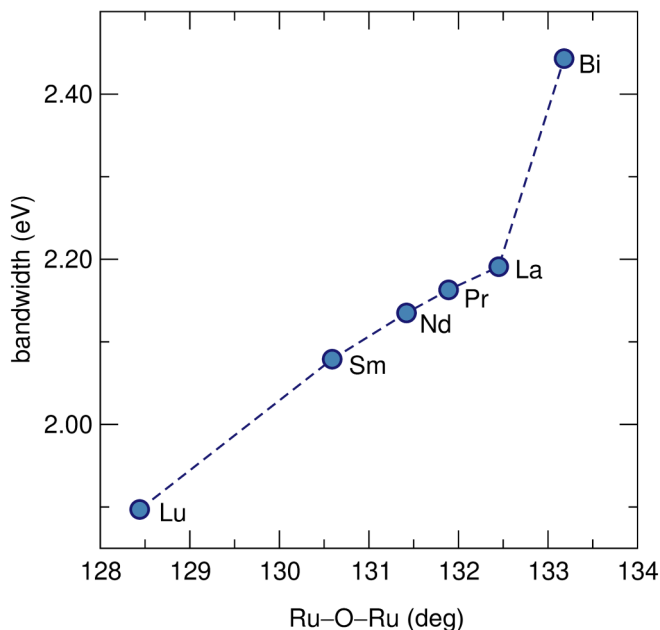
FIG. 9. Bandwidth values of the Ru t_{2g} bands as a function of the Ru-O-Ru bond angles in Ln_2Ru_2O_7 ( Ln = Lu, Sm, Nd, Pr, \text{ and } La ) and Bi_2Ru_2O_7 extracted from DFT electronic structures.
