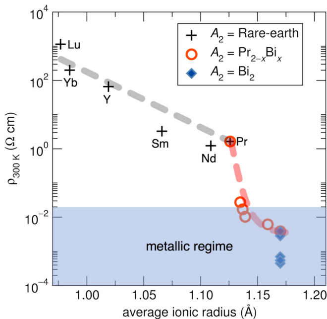
FIG. 2. Room temperature resistivity ( \rho_{300\text{K}} ) as a function of the average A -site ionic radii for the series (Pr_{1-x}Bi_x)_2Ru_2O_7 ( x = 0.0, 0.1, 0.5, \text{ and } 1.0 ), shown in open circles, illustrates a cross-over from insulating to metallic conductivity between x = 0.1 and x = 1.0 . The data is compared to literature on other A_2Ru_2O_7 pyrochlores [29,39–43] and follows expected trends.
