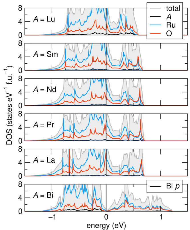
FIG. 8. Total and projected density of states (DOS) for \text{Ln}_2\text{Ru}_2\text{O}_7 ( \text{Ln} = \text{Lu}, \text{Sm}, \text{Nd}, \text{Pr}, \text{and La} ) and \text{Bi}_2\text{Ru}_2\text{O}_7 . The energies are referenced to the Fermi at 0 eV (vertical line).
