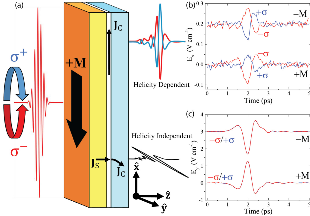
FIG. 4. (a) A schematic illustration for the laser-induced helicity-dependent and -independent photocurrent generation. The graphs on the right show the time traces of the electric field of (b) the helicity-dependent (HD) and (c) helicity-independent (HI) THz emission excited by circularly polarized ( \pm\sigma ) light. In both cases, the THz electric field can be controlled by an external magnetic field of 120 mT, which is enough to saturate the magnetization of Co. The figure shows how the reversal of the magnetization aligned along the \hat{x} axis ( \pm M ) affects the time traces of the emitted THz electric field. The curves measured for -M are shown with an offset of 0.2 V/cm for E_x in panel (b) and of 3 V/cm for E_y in panel (c).
