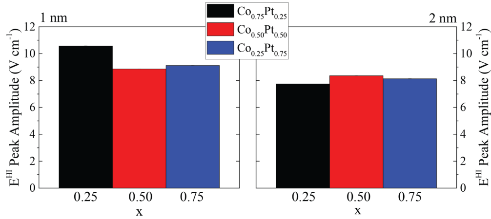
FIG. 6. The peak amplitude of the helicity-independent THz emission from samples with the \text{Co}_x\text{Pt}_{1-x} alloy spacers with thicknesses of (left panel) 1 and (right panel) 2 nm. The alloy compositions are \text{Co}_{0.75}\text{Pt}_{0.25} (black), \text{Co}_{0.50}\text{Pt}_{0.50} (red), and \text{Co}_{0.25}\text{Pt}_{0.75} (blue). The mean absolute deviation which we chose as our error bar is negligible and therefore not visible in the graph.
