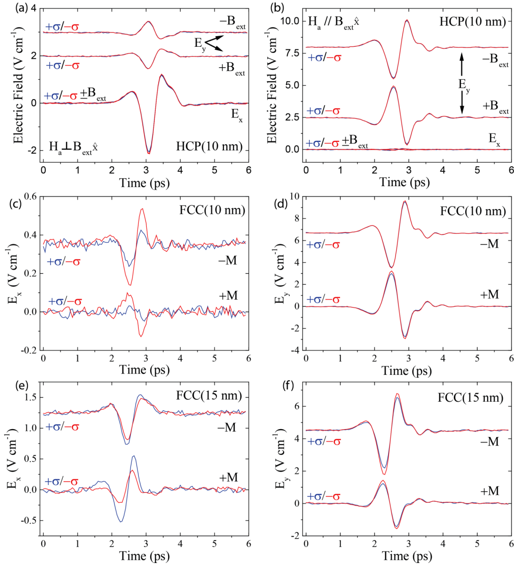
FIG. 7. Time traces of the THz electric field polarized along the \hat{x} and \hat{y} axes. The emission was generated by exciting Co/Pt bilayers with monocrystalline (hcp and fcc) Co with circularly ( +\sigma/-\sigma ) polarized laser pulses. The external magnetic field ( \pm B_{\text{ext}} ) is applied along the \hat{x} axis at 100 mT. The easy axis of the in-plane magnetic anisotropy ( H_a ) of hcp-Co is aligned either (a) perpendicular or (b) parallel to the external magnetic field. The magnetic anisotropy field strength is 0.8 T. The THz emission polarized along the \hat{x} and \hat{y} axis for (c, d) fcc-Co(10 nm) and (e, f) fcc-Co(15 nm), respectively. For fcc-Co the magnetization is saturated and is aligned parallel along the external magnetic field.
