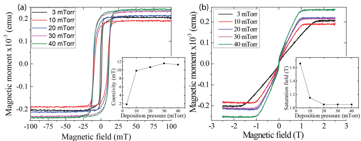
FIG. 2. (a) In-plane magnetic hysteresis loops for Co/Pt bilayers measured in Co/Pt bilayers grown at various deposition pressures of Co with the help of a vibrating sample magnetometer. (Inset) The coercive field of each hysteresis loop measured in the in-plane magnetic field. (b) The corresponding out-of-plane magnetic hysteresis loop measurements are shown. (Inset) The strength of the applied out-of-plane magnetic field corresponding to the saturation magnetization.
