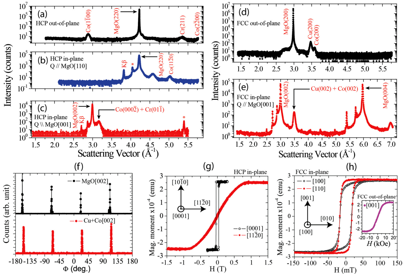
FIG. 3. The intensities of (a–e) are given in logarithmic scales. (a) The out-of-plane x-ray diffraction spectrum of the hcp-Co film. (b) The in-plane spectrum where the scattering vector \mathbf{Q} (the vector pointing along the bisection of the incoming and scattered beam) is along the MgO[110] direction, and (c) where \mathbf{Q} is along the MgO[001] direction. The x-ray diffraction spectra of (d) the out-of-plane and (e) in-plane fcc-Co film with \mathbf{Q} along the MgO[001] direction. Note that the incident x-ray angle was fixed at 0.6^\circ from the surface when the in-plane spectra was recorded. (f) \varphi scans of the MgO(002) (top) and Cu(002)+Co(002) (bottom) families of peaks. (g) In-plane magnetic hysteresis loops of (g) the hcp-Co(10 nm) and (h) fcc-Co(15 nm) film along various crystallographic directions.
