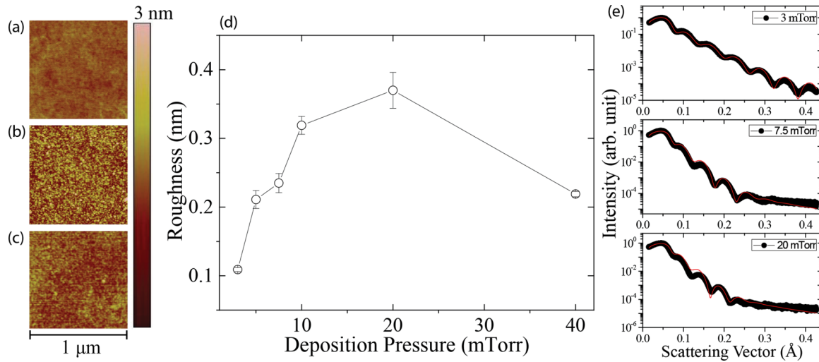
FIG. 1. AFM images of the surface of sputter-deposited pure Co films grown on glass substrates at an Ar deposition pressure of (a) 3, (b) 20, and (c) 40 mTorr. (d) AFM root-mean-square roughness of the surface of the Co films grown at various deposition pressures. (e) The x-ray reflectometry signal of Co/Pt bilayers where the Co layer was grown at deposition pressures of 3, 7.5, and 20 mTorr with the intensity plotted in logarithmic scales. The red solid curves are the fits to the experimental data.
