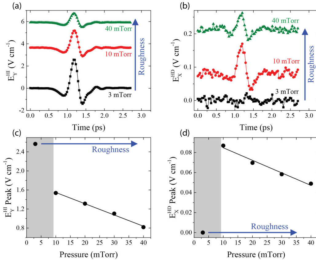
FIG. 5. (a) The helicity-independent and (b) helicity-dependent THz emission for various interfacial roughness values. The time traces are shown with a vertical offset. The observed electric field at 0 ps is 0 for the measurements. The arrows indicate the increase of the interface roughness. Peak intensities of (c) the helicity-independent THz and (d) helicity-dependent THz emission. The gray area emphasizes deviations in the behavior. Beyond the gray area ( >10 mTorr) both the helicity-independent and -dependent THz emission decreases linearly with increasing deposition pressures. The solid line is a guide to the eye.
