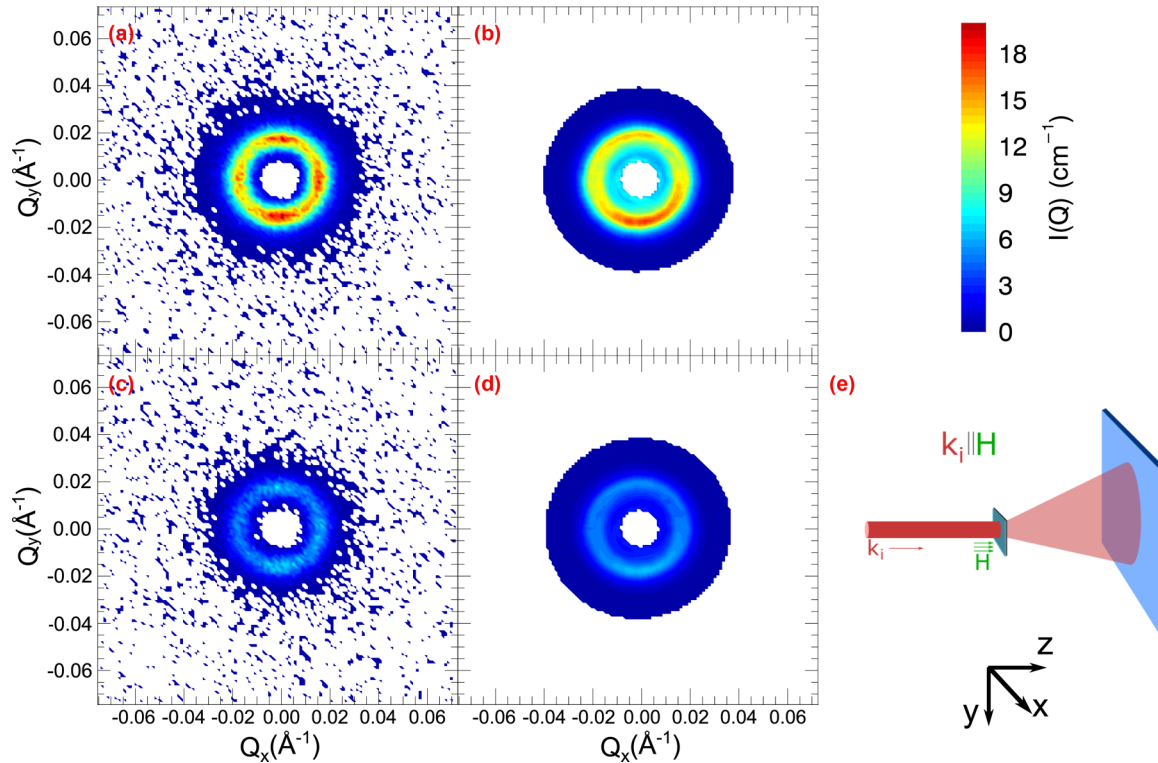
FIG. 3. SANS with polarized neutron beam for +7 mT and model fit: (a),(b) I^+(Q) , (c),(d) I^-(Q) . The ring feature is identified at Q = 0.0168 \text{ \AA}^{-1} . (e) Schematic of neutron experiment. The final wave vector k_f lies inside the cone. The scattering vector Q lies in the green colored plane at the position of the sample.
