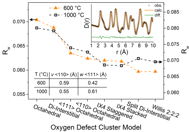
FIG. 3. Goodness-of-fit, R_w , for different defect structural models fitted to the pair distribution function, D(r) , of \text{UO}_{2.07} at 600 and 1000 °C. The IX4, split di-interstitial, and 2:2:2 Willis-type defect models yield similar fits to the experimental data, as illustrated by the low R_w values. The IX4 models yield the lowest R_w values in fitting \text{UO}_{2.07} at 1000 °C, while the split di-interstitial and Willis models yield slightly better fits to the 600 °C data. The graphical inset illustrates the fit of the Willis 2:2:2 model (red line) to the data (black circles) at 600 °C. The table inset shows the displacement values [5] for <110> and <111>-type interstitials derived from the optimized Willis 2:2:2 defect models. Dashed lines are used to guide the eye.
