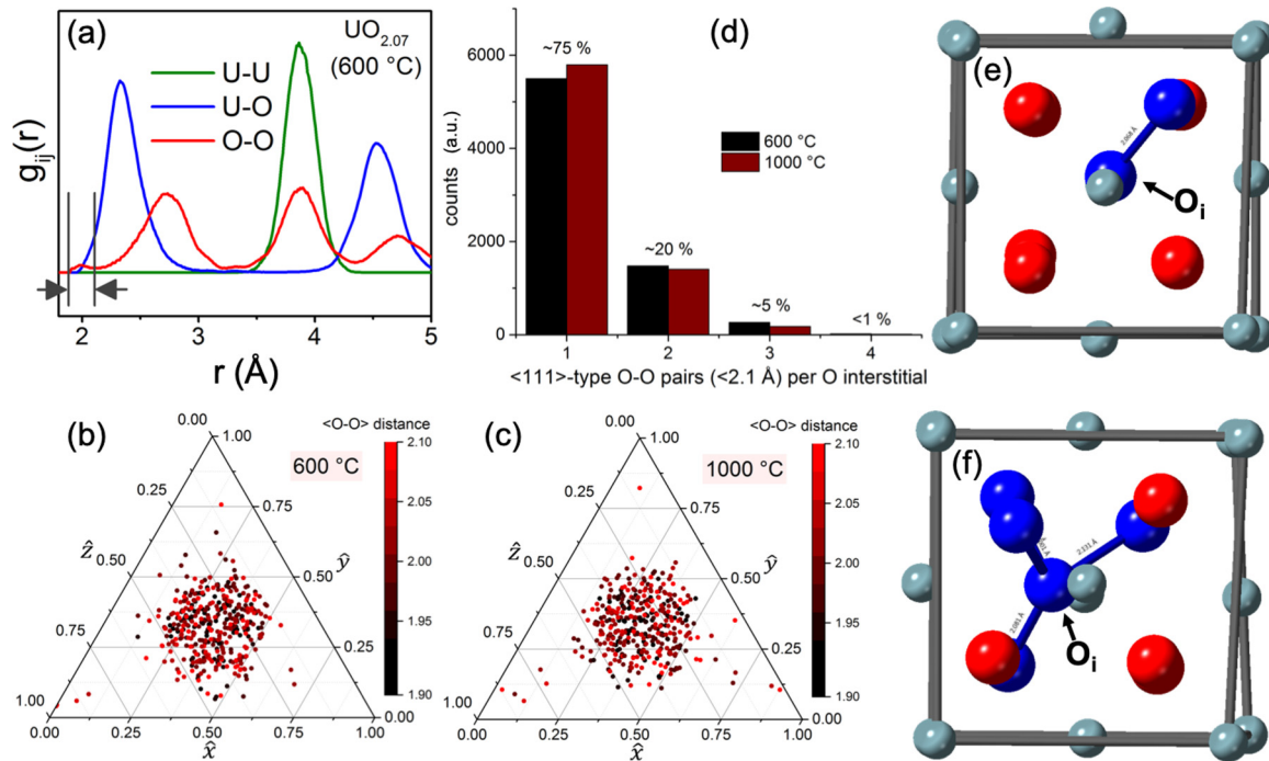
FIG. 5. Oxygen point defect configurations in \text{UO}_{2.07} reverse Monte Carlo (RMC) models at 600 and 1000 °C. (a) Oxygen interstitials in the optimized RMC models cause the emergence of a small O-O correlation at \sim 2 Å. (b),(c) Bond vector analyses show that these short (1.9–2.1 Å) O-O pairs are oriented primarily along \langle 111 \rangle directions. The edges of these ternary plots represent the three principal cubic unit vectors ( x , y , and z ), and each data point in the ternary plot represents the orientation of a single 2-Å O-O pair in an optimized RMC model. A point lying at the center of a ternary plot represents a \langle 111 \rangle O-O orientation, a point lying at one of the vertices represents a \langle 100 \rangle O-O orientation, a point lying at a leg midpoint represents a \langle 110 \rangle O-O orientation, etc. The color of the point denotes the corresponding distance for the O-O pair. (d) Counting statistics for short O-O pairs show that each interstitial forms one to four short (1.9–2.1 Å) O-O pairs with neighboring lattice oxygens. Atomic structural models for (e) single pair and (f) four-pair configurations show that oxygen interstitials are almost always located near octahedral interstitial sites and resemble monointerstitials. Uranium atoms, oxygen atoms at lattice sites, and oxygen atoms forming short O-O pairs (1.9–2.1 Å) in (e),(f) are shown in grey, red, and blue, respectively.
