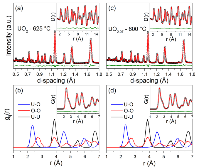
FIG. 4. Fits of optimized reverse Monte Carlo (RMC) models to experimental total scattering data of (a),(b) \text{UO}_2 at 625 °C, and (c),(d) \text{UO}_{2.07} at 600 °C. RMC models fit well to (a) and (c) long-range, (a) and (c) (insets) intermediate-range, and (b) and (d) (insets) short-range structures simultaneously. (b) and (d) \text{UO}_2 and \text{UO}_{2.07} partial pair distribution functions show similar features except for a small O-O correlation present at \sim 2 Å in the \text{UO}_{2.07} data.
