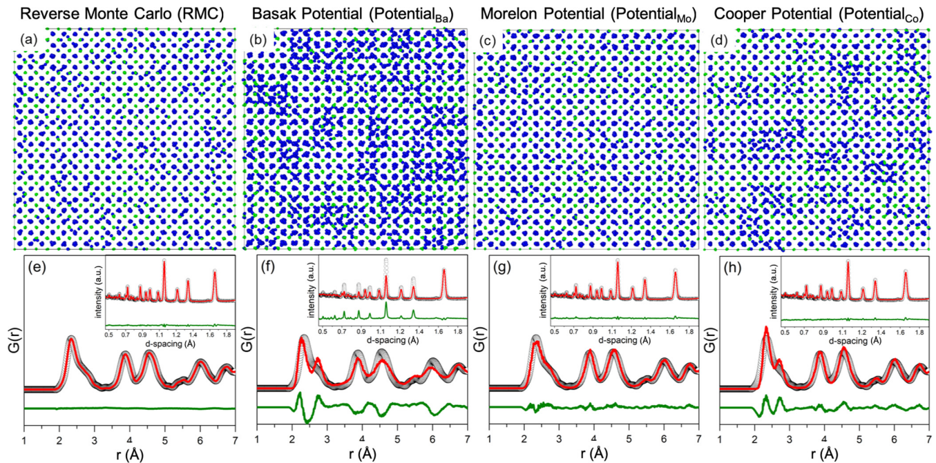
FIG. 6. Comparison of reverse Monte Carlo (RMC) and molecular dynamics (MD) models for \text{UO}_{2.07} at 600\text{ }^\circ\text{C} . (a)–(d) Projections of 10^3 optimized supercells along principal axes. Uranium and oxygen atoms are shown in green and blue, respectively. (e)–(h) Comparisons of simulated PDFs (red lines) with experimental PDFs (black circles), and difference curves (green lines). Insets of (e)–(h) show simulated Bragg patterns (red lines), experimental Bragg patterns (black circles), and difference curves (green lines). MD Potential Ba yields the most disordered structural models that poorly reproduce all experimental data. Potential C o models are less disordered and contain larger defect clusters, but do not adequately reproduce the experimental PDF at low r values. Potential M o models contain small point defects, are qualitatively similar to the RMC model, and best reproduce all experimental data, as illustrated by the low-intensity difference curves.
