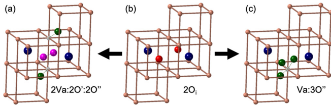
FIG. 1. Select oxygen defect cluster morphologies proposed to exist in single-phase \text{UO}_{2+x} by various researchers. Simple-cubic oxygen sublattices are shown in brown and lattice uranium atoms are shown as blue spheres. (b) A simple di-interstitial cluster comprises two neighboring octahedral interstitials separated along a \langle 110 \rangle direction (red spheres). (a) These octahedral interstitials can displace along \langle 110 \rangle directions (pink spheres; O' -type interstitials) and displace two neighboring lattice oxygens along \langle 111 \rangle directions (green spheres; O'' -type interstitials) to form a so-called 2:2:2 Willis-type defect cluster. (c) Alternatively, octahedral interstitials can displace along \langle 111 \rangle directions (green spheres) and displace a neighboring lattice oxygen along a \langle 111 \rangle direction (green sphere) to form a split di-interstitial cluster. Split di-interstitial clusters can further chain together in pairs to form split quad interstitial (IX4) defects or agglomerate in larger numbers to form larger cuboctahedral defects with occupied or unoccupied centers.
