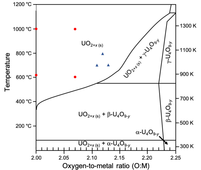
FIG. 2. Phase diagram of uranium oxide at ambient pressure adapted from Ref. [37]. \text{UO}_{2+x(s)} denotes the single-phase hyperstoichiometric regime. Red dots indicate temperatures and O:M values at which neutron total scattering measurements were performed. Blue triangles illustrate the region investigated by Willis and Murray using single-crystal neutron diffraction [4,5].
