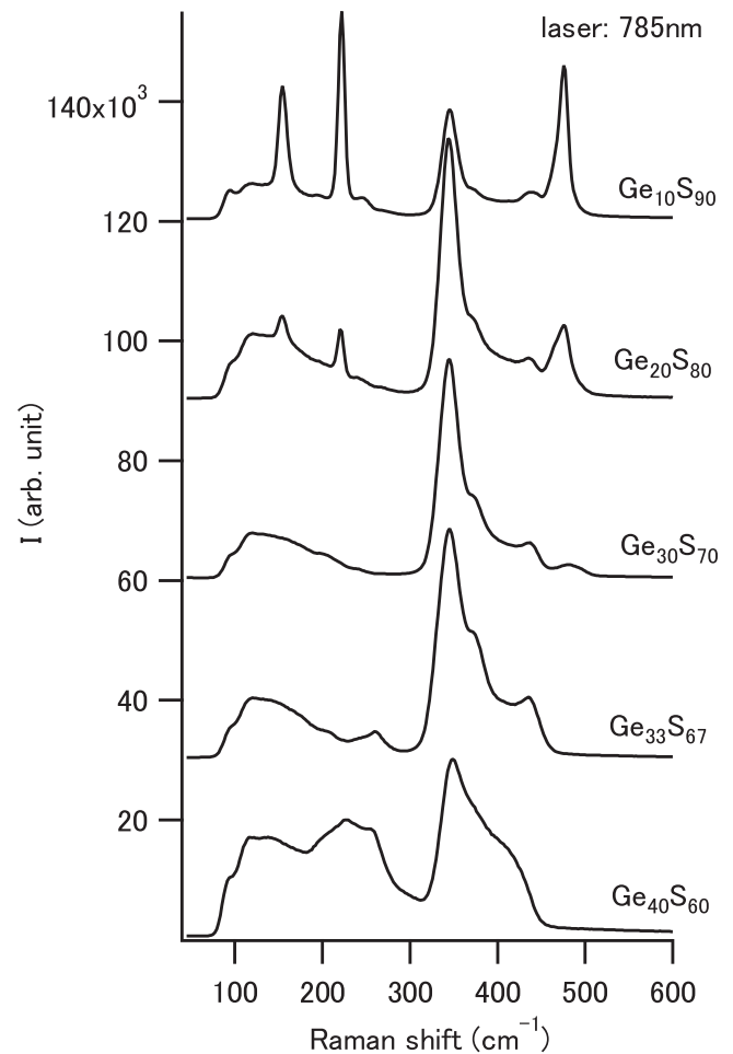
FIG. 22. Raman spectra of \text{Ge}_x\text{S}_{100-x} ( x = 10, 20, 30, 33, 40 ) glasses using the excitation laser with the wavelength of 785 nm.
