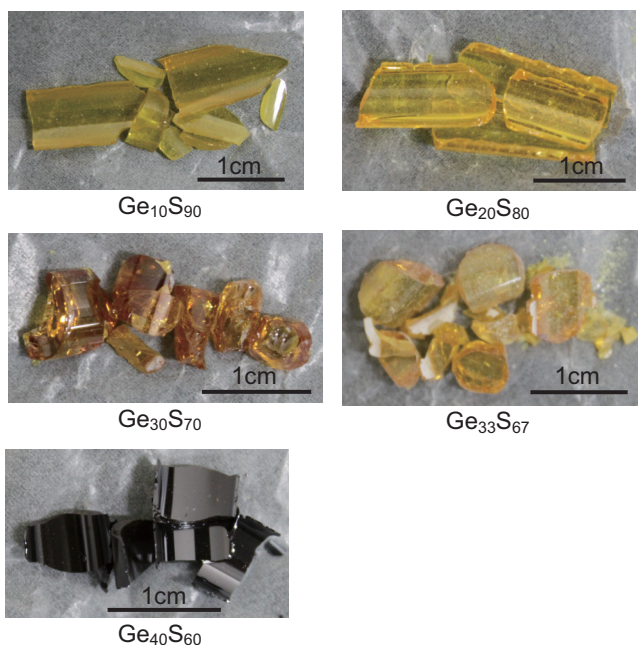
FIG. 6. Colors of Ge-S glasses.
