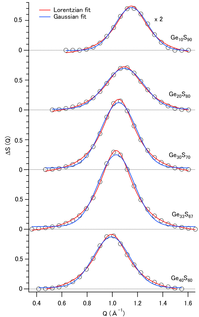
FIG. 17. Curve fitting to the net FSDP curve using the Lorentzian and Gaussian. The net FSDP curves were obtained by subtracting the base curve (the broken curve in Fig. 15) from the experimental curve in Fig. 15. The curve for \text{Ge}_{10}\text{S}_{90} is multiplied by 2.
