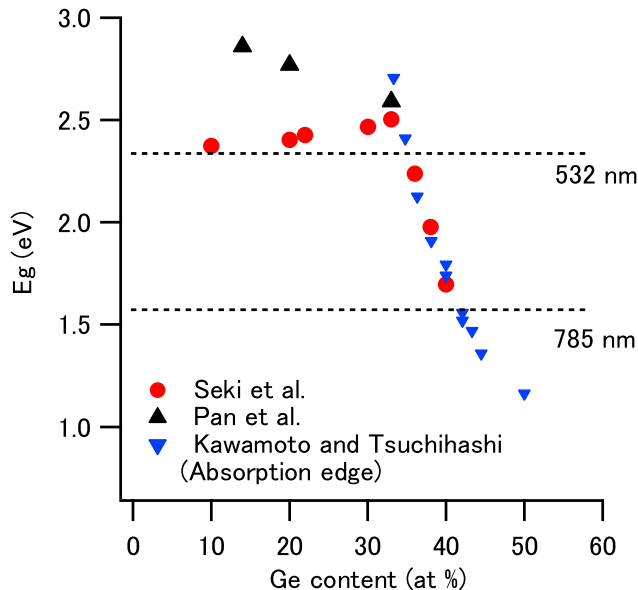
FIG. 5. Composition dependence of the optical gap of Ge-S glasses. Red circles indicate the data measured by Seki et al. [56] and the black triangles indicate the data measured by Pan et al. [57]. The optical absorption edges measured by Kawamoto and Tsuchihashi [58] are also shown in blue triangles. The broken lines indicate the energies of the excitation lasers used for Raman scattering measurement, which will be discussed in Sec. III B.
