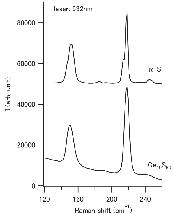
FIG. 23. Comparison of Raman spectra of \alpha sulfur and \text{Ge}_{10}\text{S}_{90} glasses, ranging from 120 to 250 \text{ cm}^{-1} .
