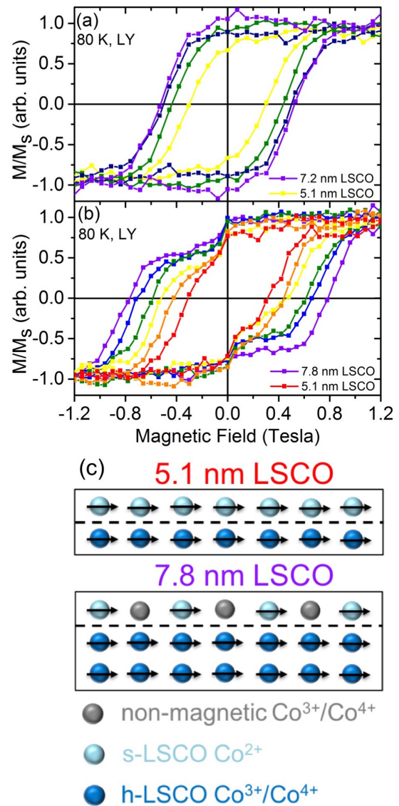
FIG. 4. Major LY Co-XMCD hysteresis loops in from (a) the single layer LSCO wedge and (b) the LSCO wedge bilayer. (c) Proposed structure of the magnetic interface between s-LSCO and h-LSCO at the two endpoints of the bilayer.
