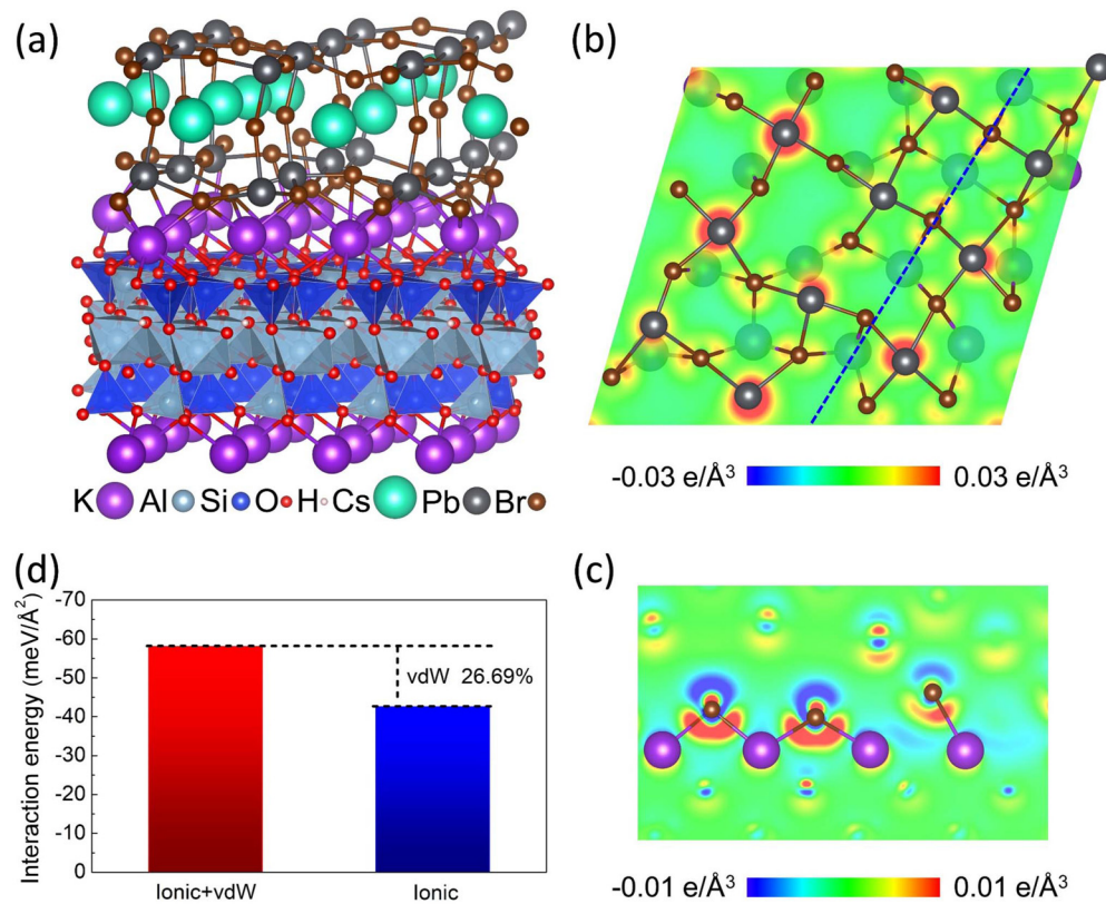
FIG. 4. DFT simulation of the interfacial interaction between the epitaxial halide perovskite \text{CsPbBr}_3 and the mica substrate. (a) Atomistic model of the relaxed supercell used in DFT calculations. The atoms have been labeled and drawn to their relative sizes. (b) The planar view of atomic stacking and charge transfer at the \text{CsPbBr}_3 /mica interface. (c) Cross section noted as the blue dashed line in (b), and a significant charge transfer between the potassium and the bromine atoms can be observed. (d) Calculation of the interaction energy at the interface that with and without vdW interactions. The vdW interaction takes a significant portion of the overall interaction energy, meaning a relatively strong vdW force.
