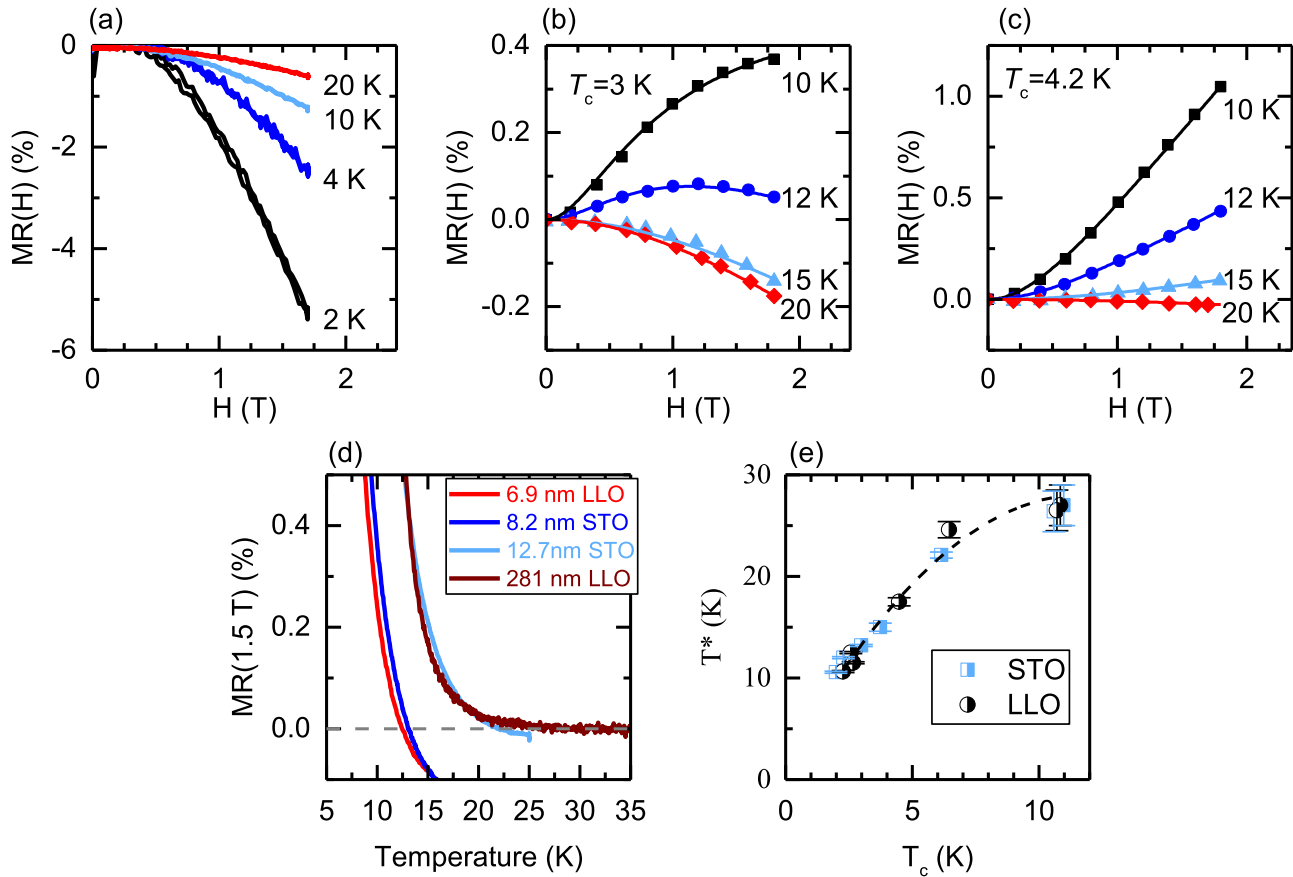
FIG. 5. Magnetoresistance measurements above T_c . Magnetoresistance at fixed temperatures for (a) insulating 5.5 nm on STO, (b) superconducting 8.2 nm BPBO on STO, and (c) superconducting 7.8 nm BPBO on LLO. In (b) and (c) the markers are experimental data points with the solid lines fits to superconducting fluctuations and weak localization in a 2D disordered system. (d) Representative magnetoresistance vs temperature. (e) The MR inflection temperature T^* vs T_c (the dashed line is a guide for the eye).
