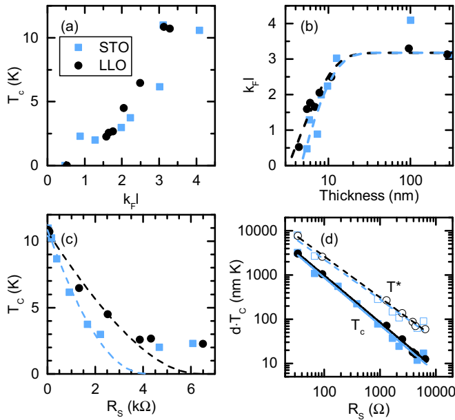
FIG. 3. Disorder and superconductivity. (a) Transition temperature vs the Mott-Ioffe-Regel parameter, k_F l (extracted from room temperature measurements), and (b) k_F l vs thickness (the dashed lines are guides for the eye). (c) T_c vs the sheet resistance at 20 K. The dashed lines are fits to Finkel'stein's model for a homogeneously disordered superconductor. (d) Power-law scaling dependence of thickness times transition temperature ( d \times T_c ) versus R_s based on the phenomenological formula d \times T_c = AR_s^{-B} , where A and B are fitting parameters [31].
