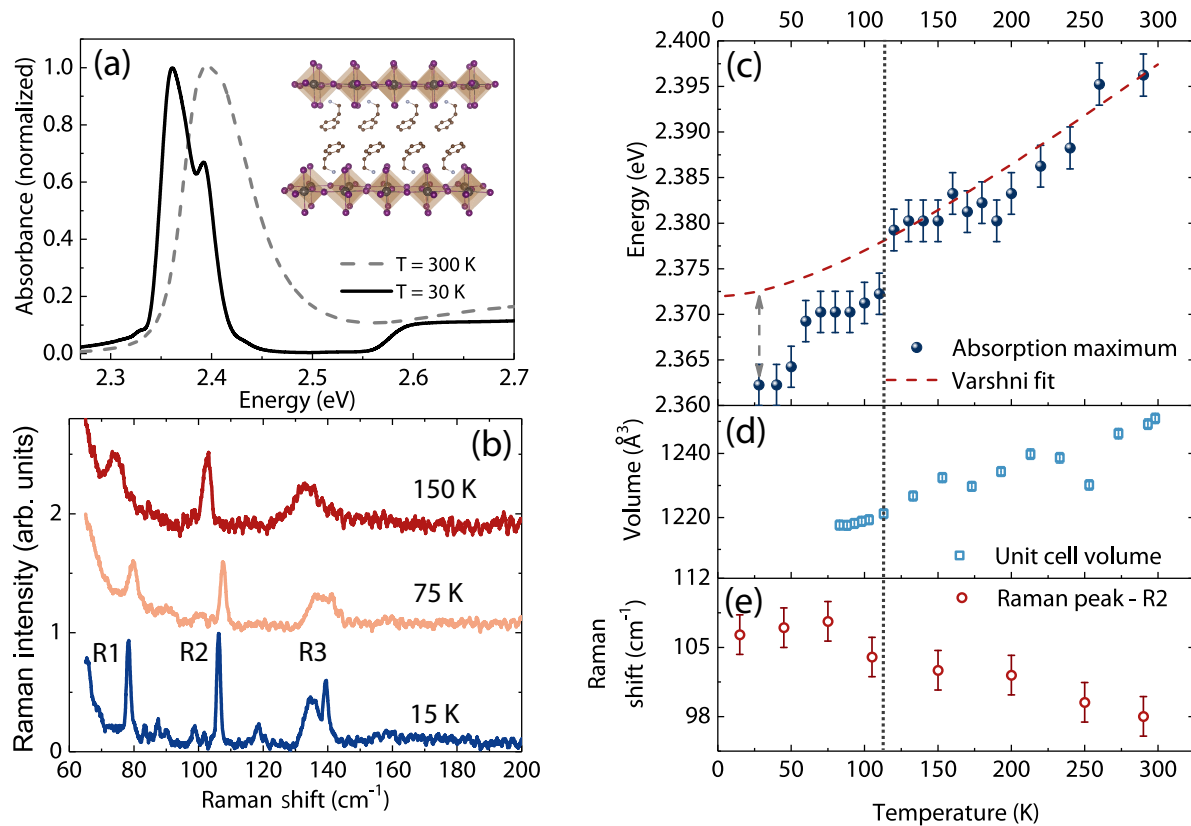
FIG. 1. The relationship between optical and structural properties of (\text{PEA})_2\text{PbI}_4 . (a) Absorption spectra and structure (inset) of (\text{PEA})_2\text{PbI}_4 monolayer 2D perovskite at low (30 K) and room (300 K) temperature. (b) Nonresonant Raman spectra of the sample taken at three different temperatures. The main modes identified within this range are labeled as R1, R2, R3. (c) Position of the excitonic peak in the absorption spectrum, plotted as a function of the temperature. Also shown as a dotted line is a Varshni fit of the trend, assuming temperature independence of the exciton binding energy. (d) Unit-cell volume estimated from the wide-angle x-ray scattering data shown at various temperatures. (e) Position of the peak R2 in the Raman spectrum plotted at different temperatures. The uncertainty bars represent instrument resolution.
