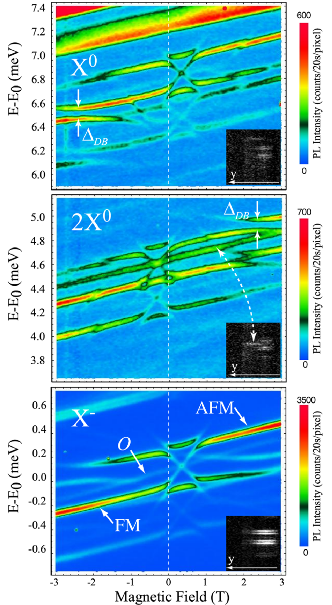
FIG. 2 (color online). Contour plot of \mu -PL intensity from a single InAs QD doped with a single Mn impurity against longitudinal magnetic field and detection energy E - E_0 ( E_0 = 1.2536 eV). The three energy windows correspond to the X^0 , 2X^0 , and X^- states observed in the same \mu -PL spectra. Insets: CCD images ( 100 \text{ pixels} \times \sim 150 \text{ pixels} ) at B_z = 0 T showing the spatial correlations of the lines along the vertical axis y of the setup. An extra line coming from another QD (dashed arrow) is superposed on the 2X^0 feature.
