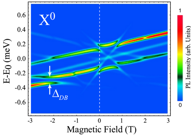
FIG. 3 (color online). Theoretical contour plot of X^0 PL intensity from a single InAs QD doped with a single Mn impurity against longitudinal magnetic field and energy.
