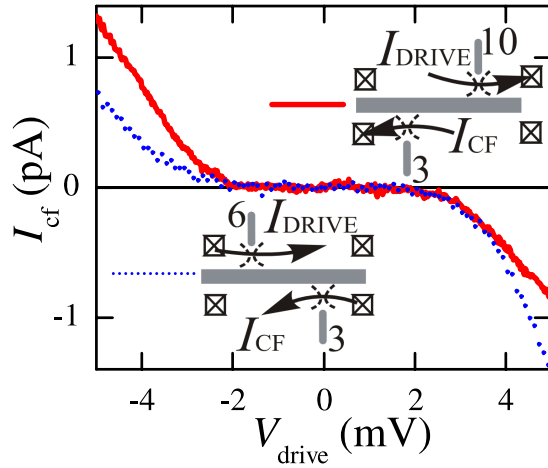
FIG. 4 (color online). Drive bias dependence of the counterflow current through the pinched-off detector QPC for the drive QPC formed with gate 6 (dotted line) or gate 10 (solid line). The detector QPC conductance is about G_{\text{det}} = 5 \text{ G}\Omega^{-1} . The drive QPCs are tuned to provide the maximal effect. Insets: sketches of the two counterflow measurements. The directions of currents are shown for the case of V_{\text{drive}} > 0 .
