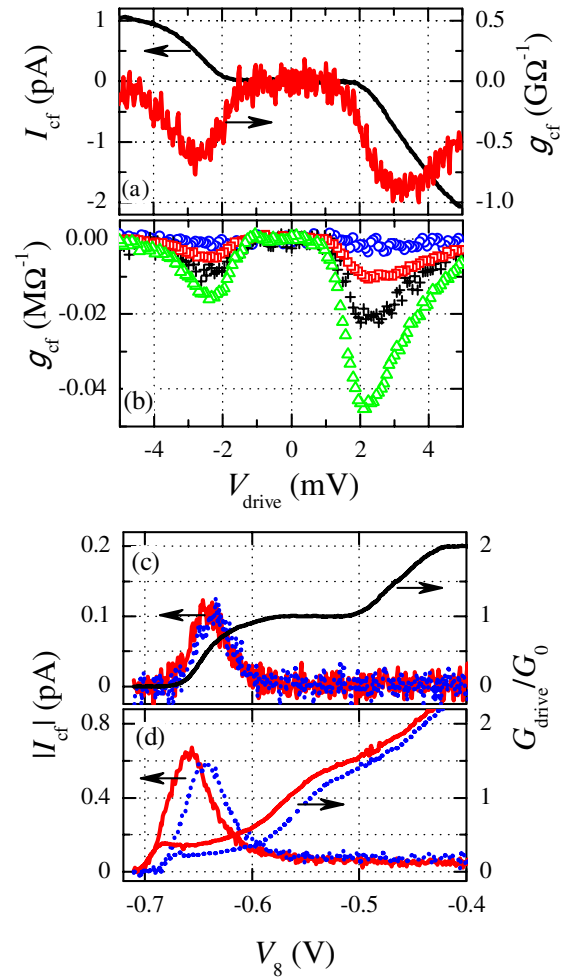
FIG. 2 (color online). (a) I_{\text{cf}} and g_{\text{cf}} for the nearly pinched-off detector QPC as a function of V_{\text{drive}} . (b) g_{\text{cf}} measured for a set of G_{\text{det}} values marked by according symbols in Fig. 1. (c),(d) Absolute value of I_{\text{cf}} as a function of the drive QPC gate voltage V_8 , for V_{\text{drive}} = \pm 2.25 mV (c) and V_{\text{drive}} = \pm 4 mV (d). Also shown is the drive QPC's conductance in linear response (c) and its differential conductance at V_{\text{drive}} = \pm 4 mV (d). Solid (dotted) lines correspond to V_{\text{drive}} < 0 ( > 0 ). In (a),(b) gates 7 and 9 are grounded, while in (c),(d) V_7 = V_9 = -0.4 V. The drive bias modulation used to measure g_{\text{cf}} is 92 \mu\text{V} rms.
