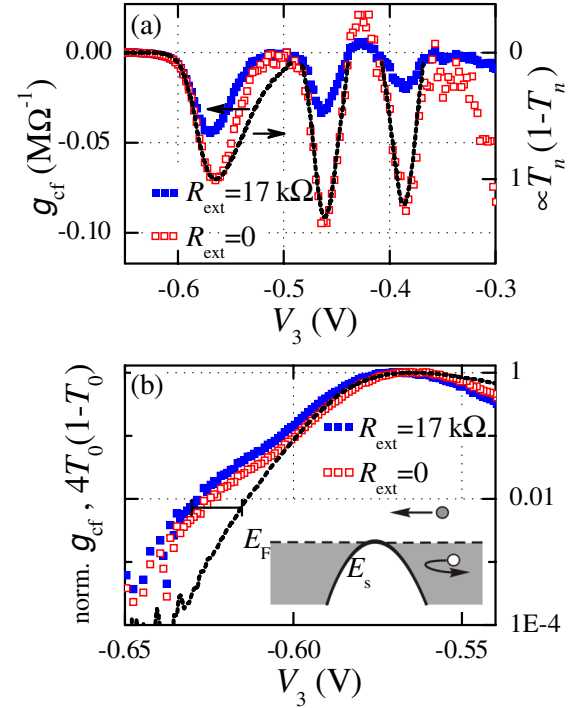
FIG. 3 (color online). (a) g_{cf} as a function of the detector QPC gate voltage V_3 . Closed symbols correspond to the g_{cf} measured at a finite external resistance R_{ext} = 17 k \Omega , while open symbols show the corrected counterflow conductance R_{ext} = 0 (see text). Also shown are the transmission functions T_n(1 - T_n) for the three lowest 1D subbands of the detector QPC (dashed lines), scaled to fit the corrected data. During the g_{cf} measurement the drive bias is modulated with a 230 \mu V rms signal about the mean value V_{drive} = +2.05 mV. (b) Normalized g_{cf} [symbols as in (a)] and transmission function of the lowest 1D detector QPC subband 4T_0(1 - T_0) (dashed line) as a function of V_3 . The scale bar shows a gate voltage interval corresponding to a change of the 1D subband energy by 0.5 meV. Inset: Sketch of possible scattering processes of nonequilibrium electrons and holes at a partially transmitting detector QPC.
