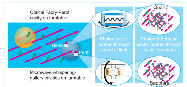
FIG. 1 (color online). Modifications of c , n , and L are probed for cavities of different geometry and material, which allows us to separately probe Lorentz violation in the electron and photon sector (symbolized by the arrows).
